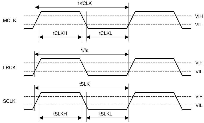
Clock Timing
