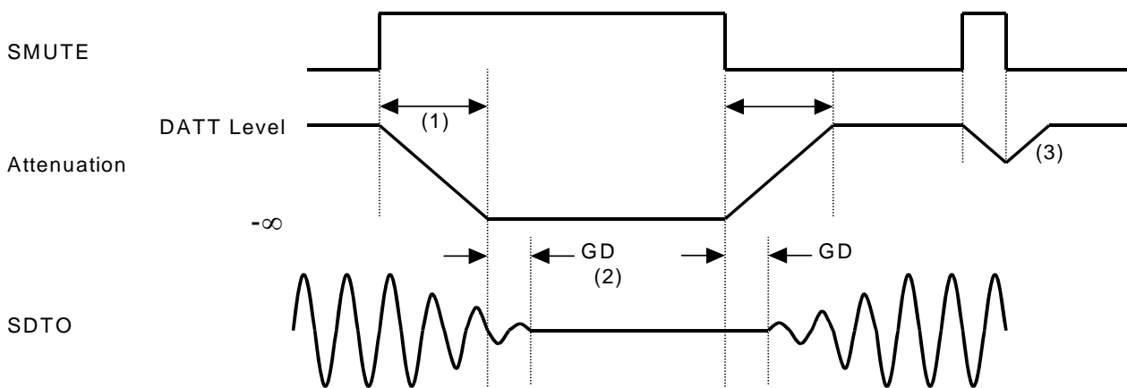
Figure 13. Soft Mute Function
