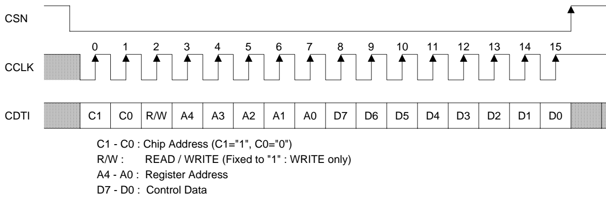
Figure 14. Serial Control I/F Timing
