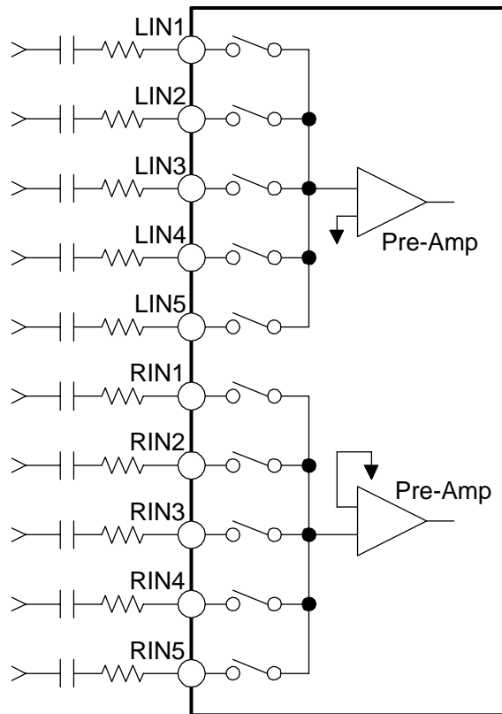
Figure 5. Input Selector
