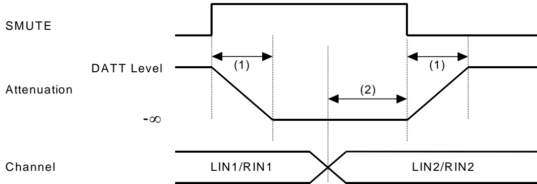
Figure 6. Input channel switching sequence example
