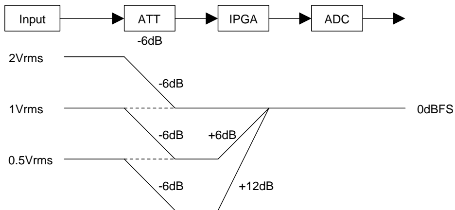
Figure 9. ALC Level diagram example (ALC=OFF)
