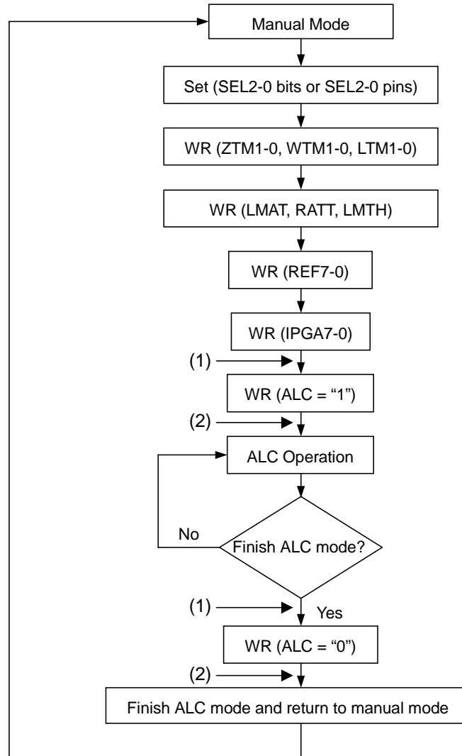
Note : WR : Write Figure 12. Registers set-up sequence at ALC operation
