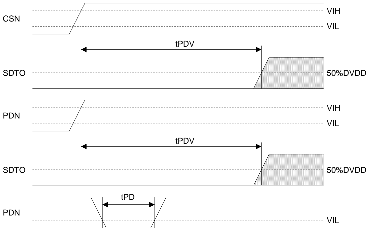
Power Down & Reset Timing
