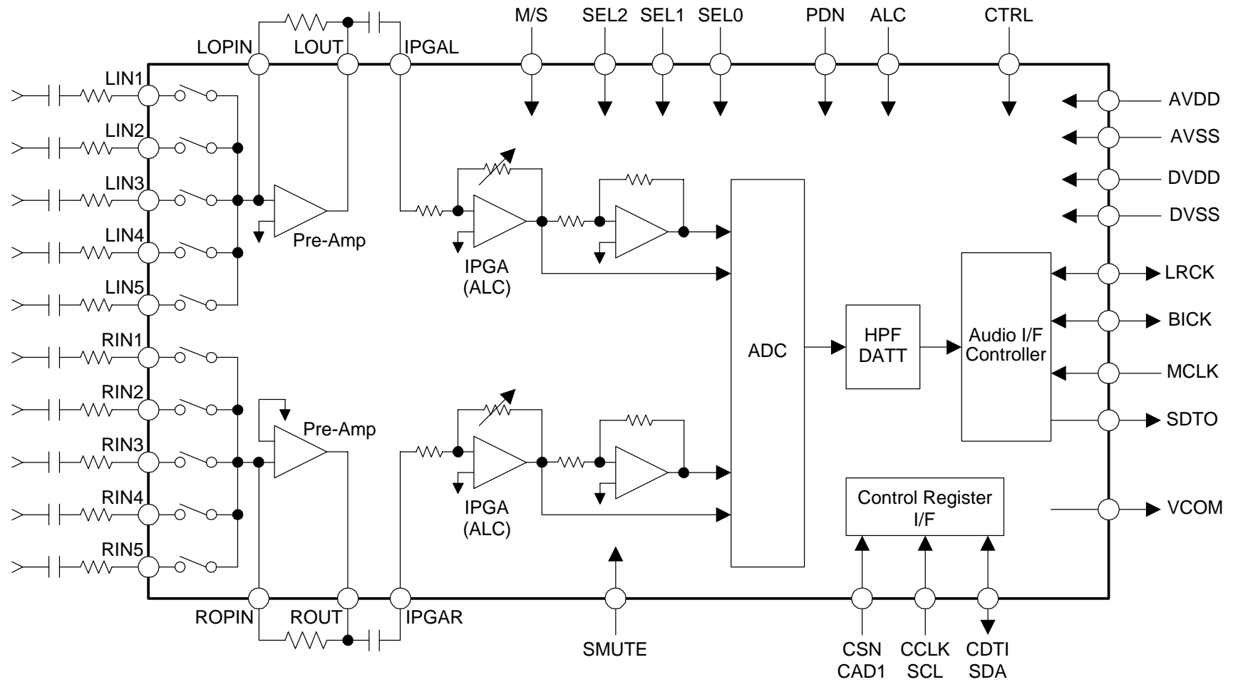
Block diagram
