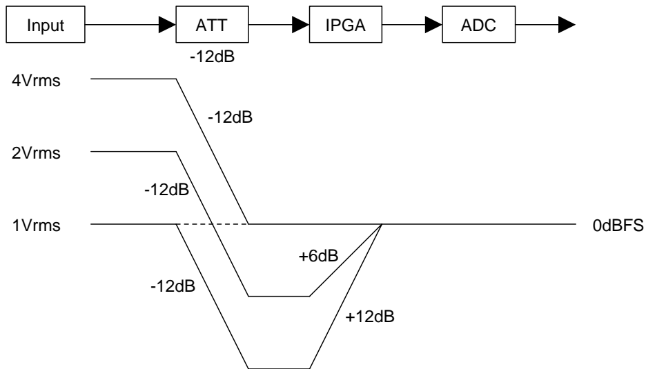
Figure 8. ALC Level diagram example (ALC=OFF)
