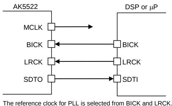
Figure 34. PLL Slave Mode
