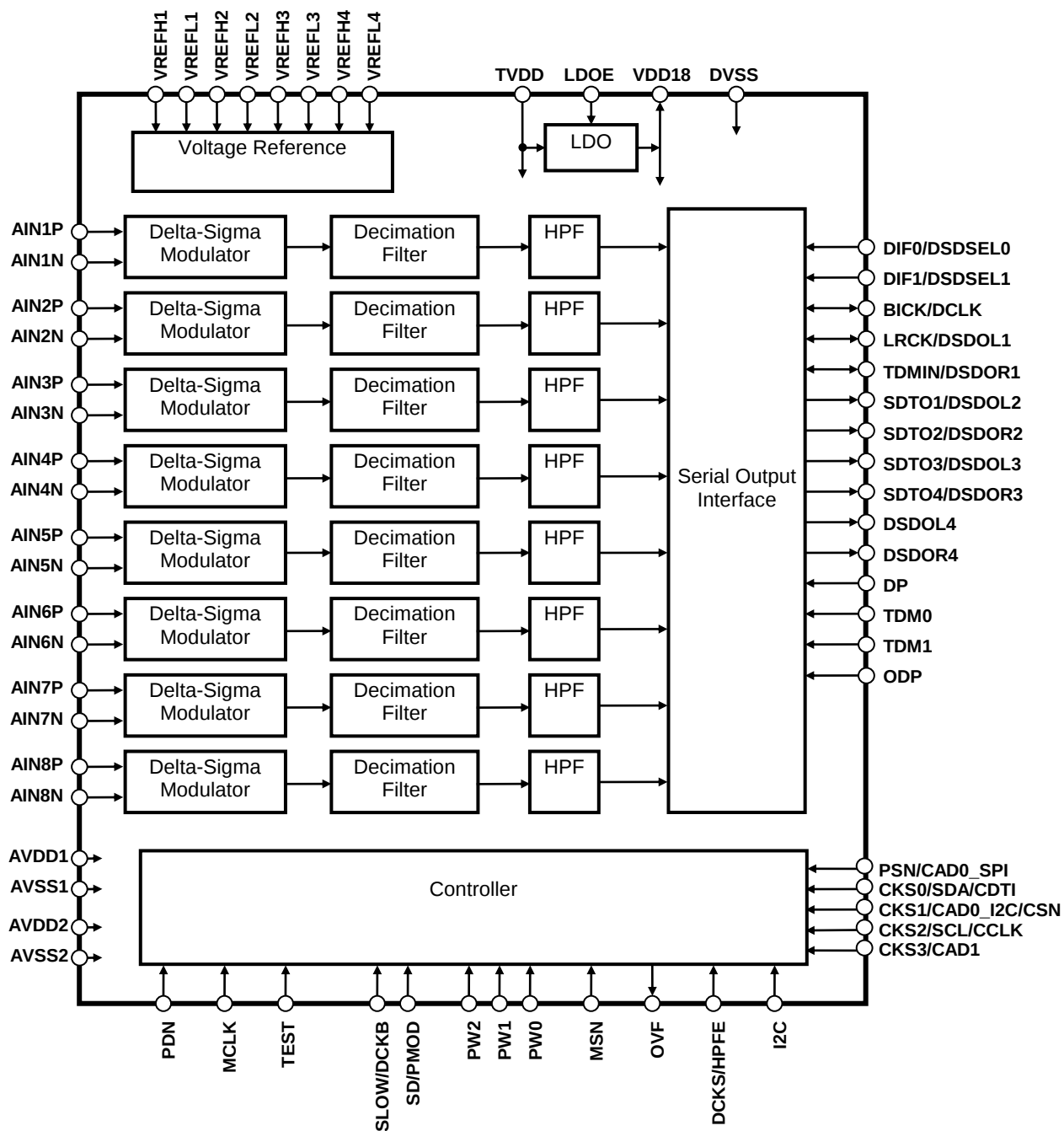
Figure 1. Block Diagram
