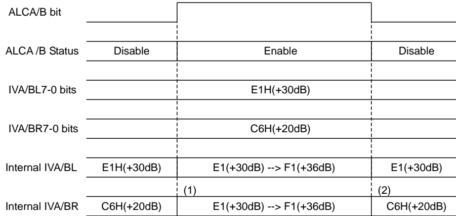
Figure 44. IVOL value during 2ch ALC operation
