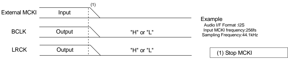
Figure 69. Clock Stopping Sequence (5)
