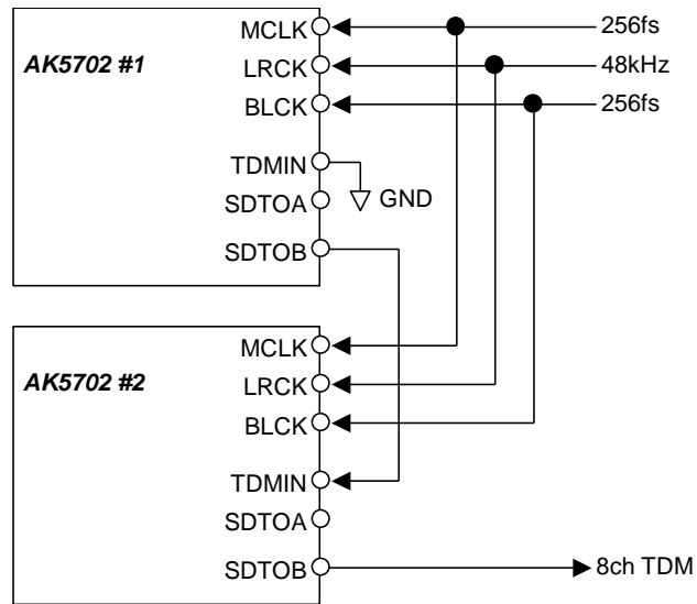
Figure 37. Cascade TDM Connection example (TDM256, MSB justified)
