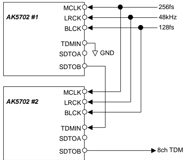
Figure 35. Cascade TDM Connection example (TDM128, MSB justified)
