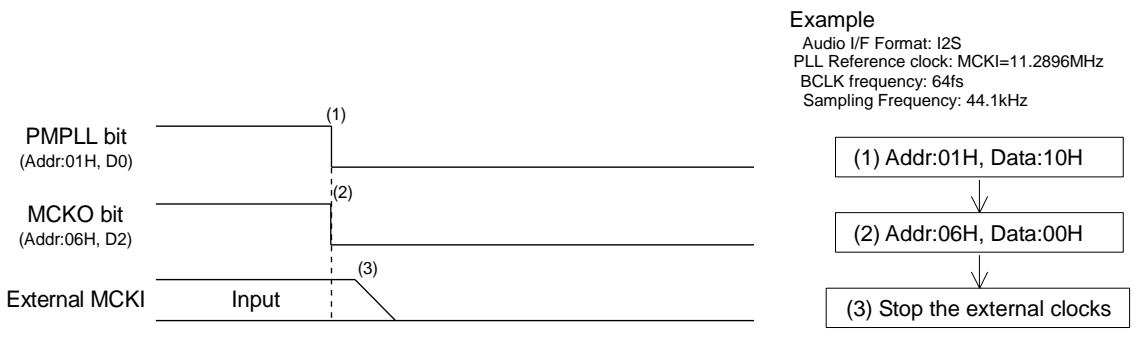
Figure 67. Clock Stopping Sequence (3)
