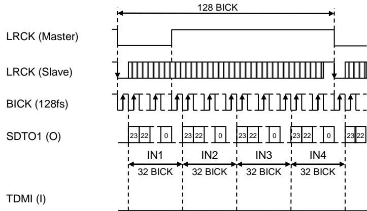
Figure 31 Mode 2 Timing (TDM128 Mode, 24-bits I 2 S Compatible)
