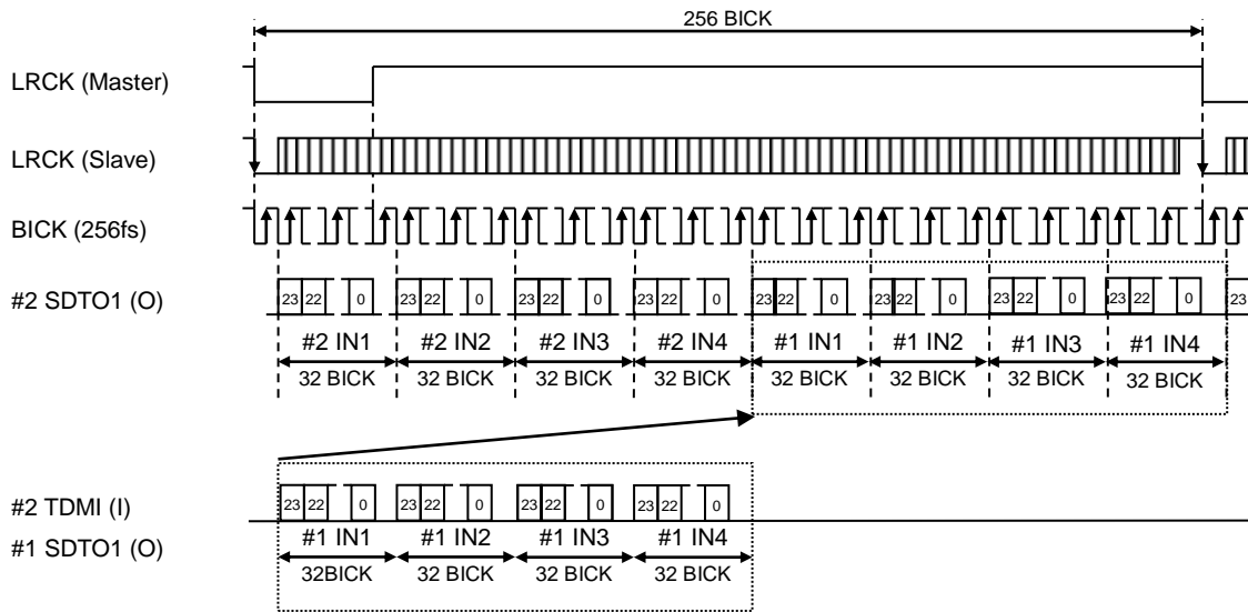
Figure 35. Mode 6 Timing (TDM256 Mode, 24-bits I²S Compatible)
