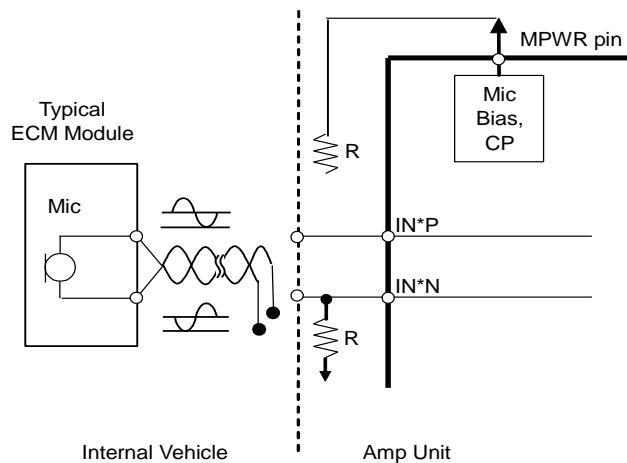
Figure 56: Negative Input OPEN
