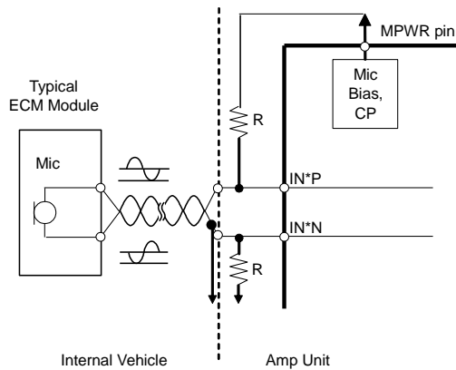
Figure 60: Negative Input Short to GND
