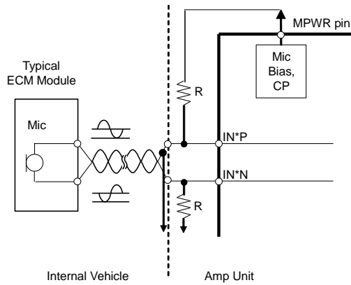
Figure 59: Positive Input Short to GND
