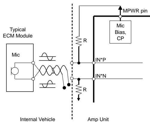
Figure 54: Positive and Negative Input OPEN
