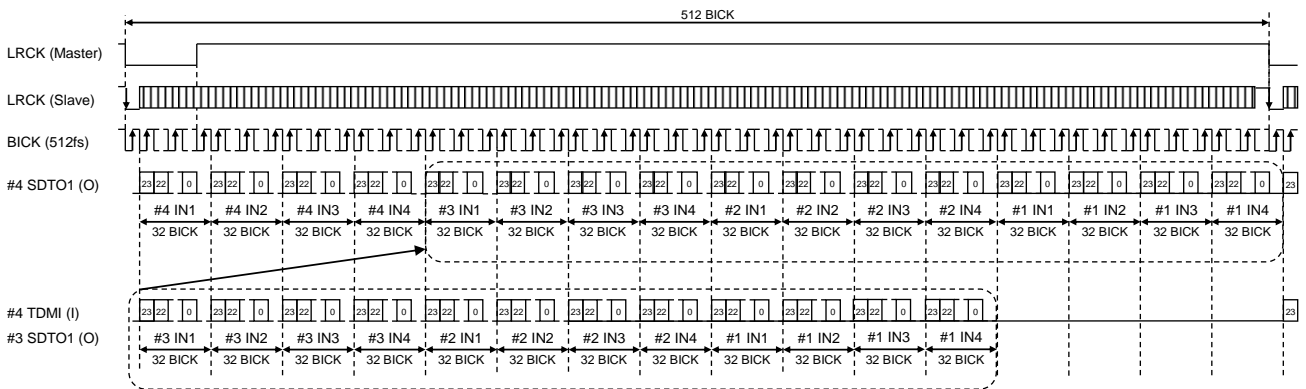
Figure 39. Mode 10 Timing (TDM512 Mode, 24-bits I 2 S Compatible)
