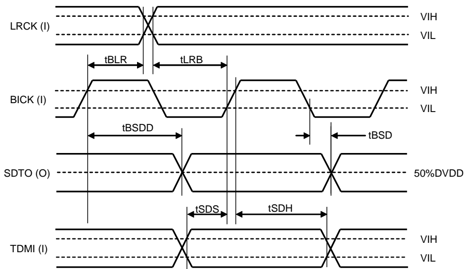
Figure 19. Audio Interface Timing (TDM mode & Slave mode)
