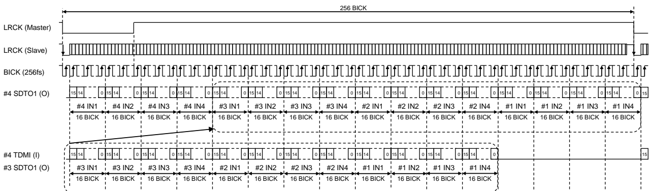
Figure 37. Mode 8 Timing (TDM256 Mode, 16-bit I²S Compatible)
