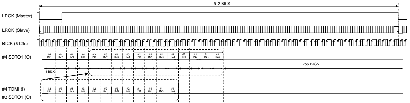
Figure 41. Mode 12 Timing (TDM512 Mode, 16-bits I 2 S Compatible, 1 SLOT = 16 BICK)
