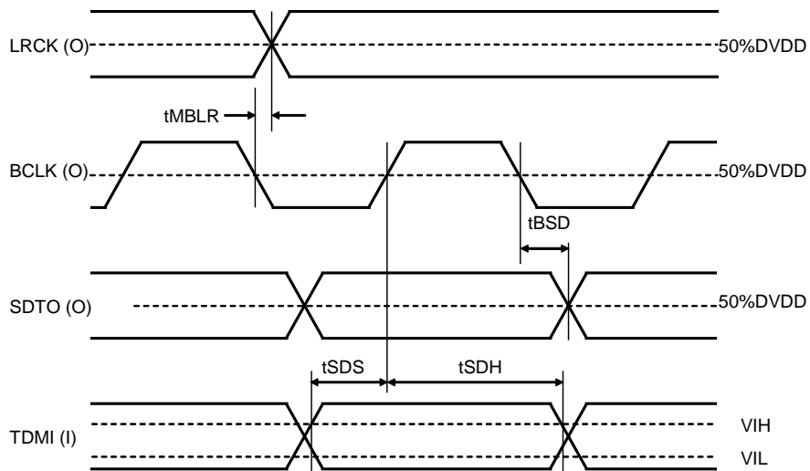
Figure 20. Audio Interface Timing (TDM mode & Master mode)
