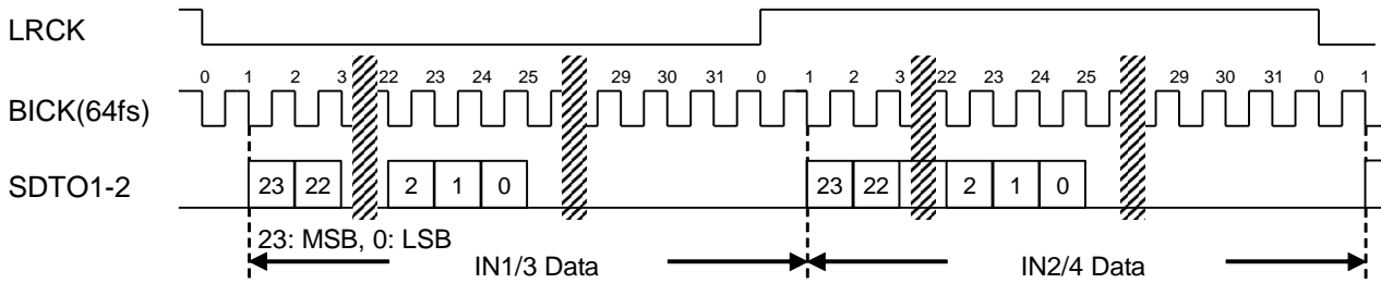
Figure 29. Mode 0 Timing (Stereo Mode (24-bits I 2 S))
