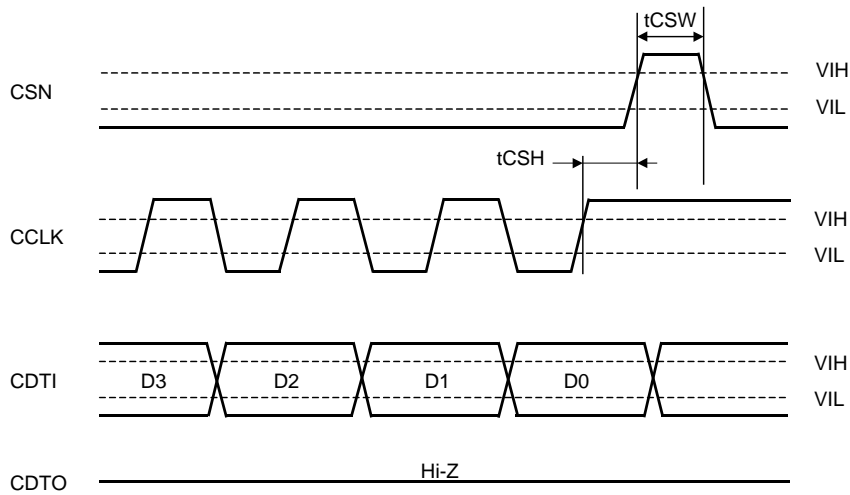
Figure 23. WRITE Data Input Timing (4-wire serial mode)
