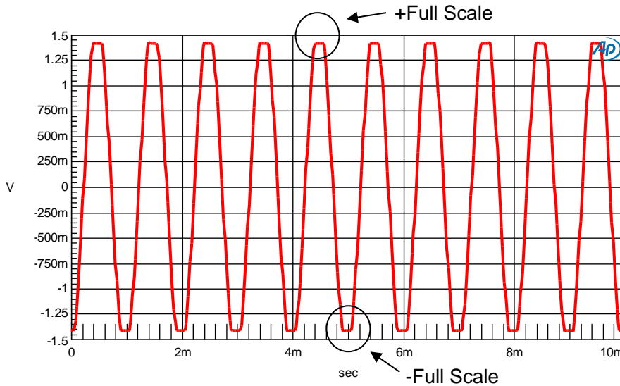
Figure 50: Output Signal with an input of 1kHz 2.3Vrms Signal (2.0Vrms = 0dBFS)
