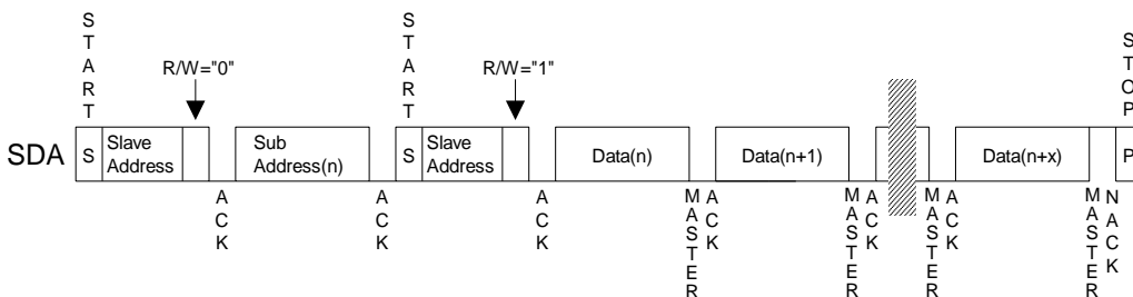
Figure 71: Random Address Read
