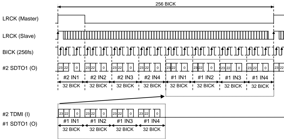
Figure 36. Mode 7 Timing (TDM256 Mode, 24-bit MSB Justified)
