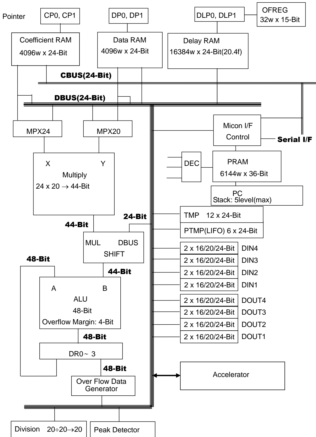
Figure 2. AK7736B Main DSP Block Diagram
