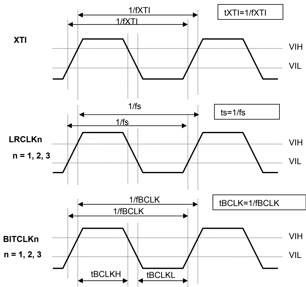
Figure 4. System Clock
