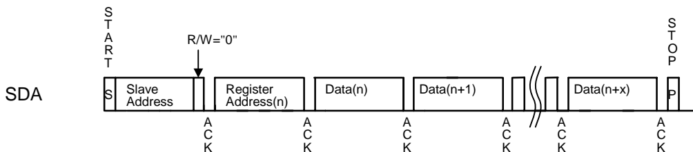
Fig. 07 WRITE Operation
