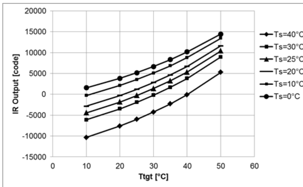
Figure 18.1. IR Output
