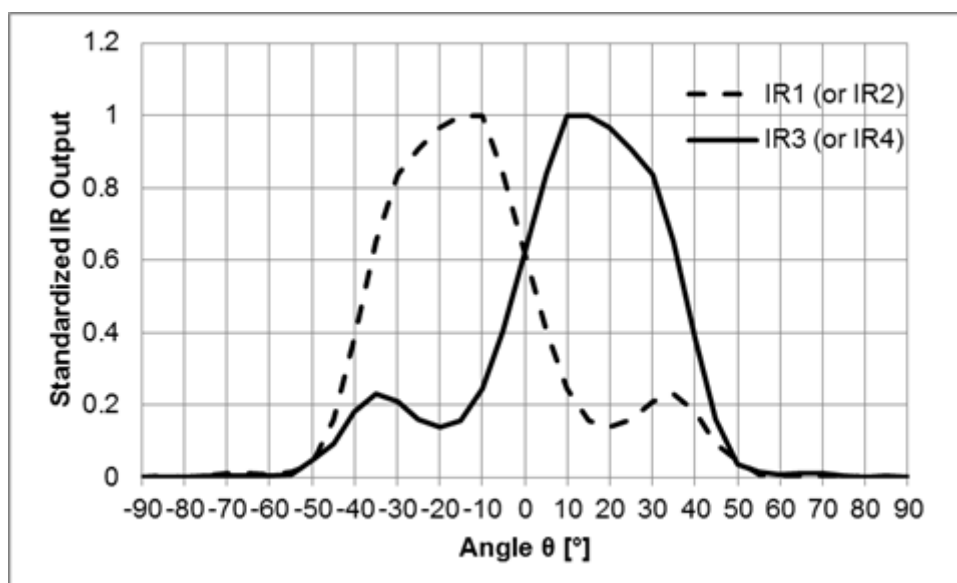
Figure 20.1. Field of View (Typ.)
