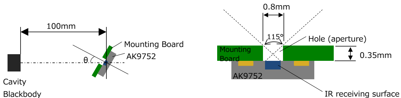
Figure 15.2. Measurement environment
