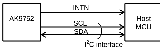
Figure 10.1 Example of use (Connection diagram)
