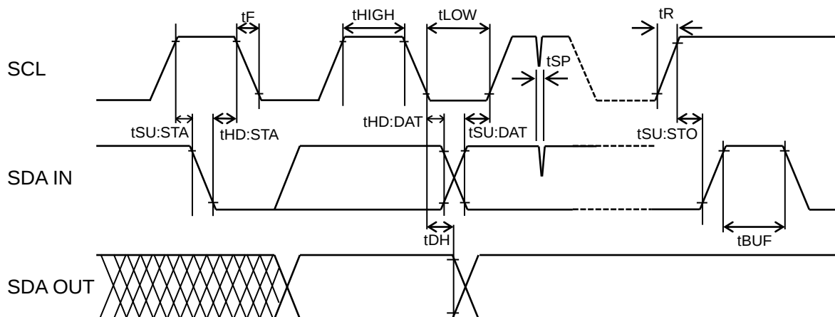
Figure 9.1 Bus Timing
