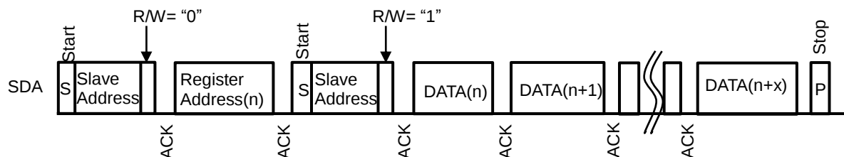
Figure 11.9. Random Read
