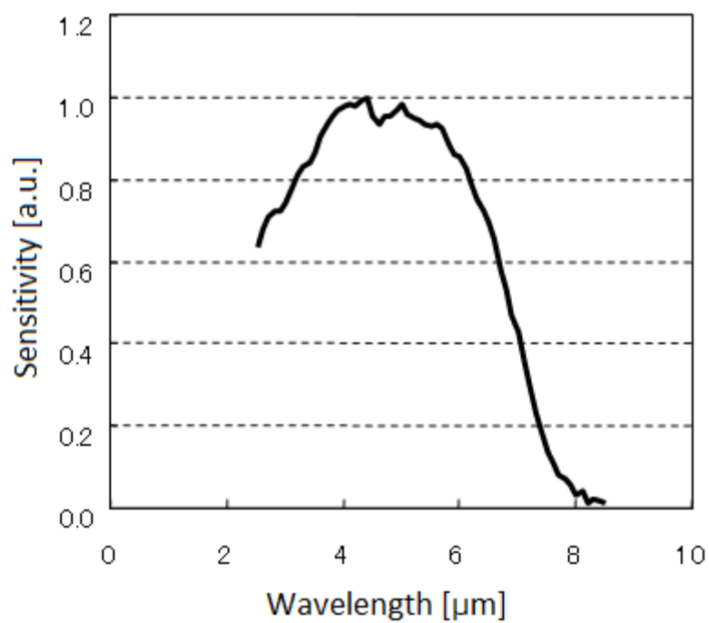
Figure 14.1. Spectrum Sensitivity
