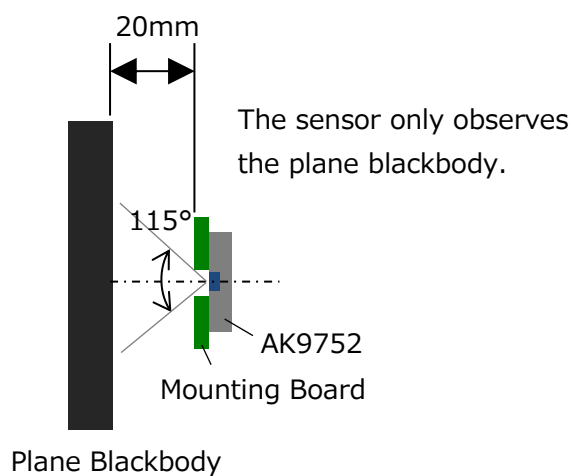
Figure 16.2. Measurement environment
