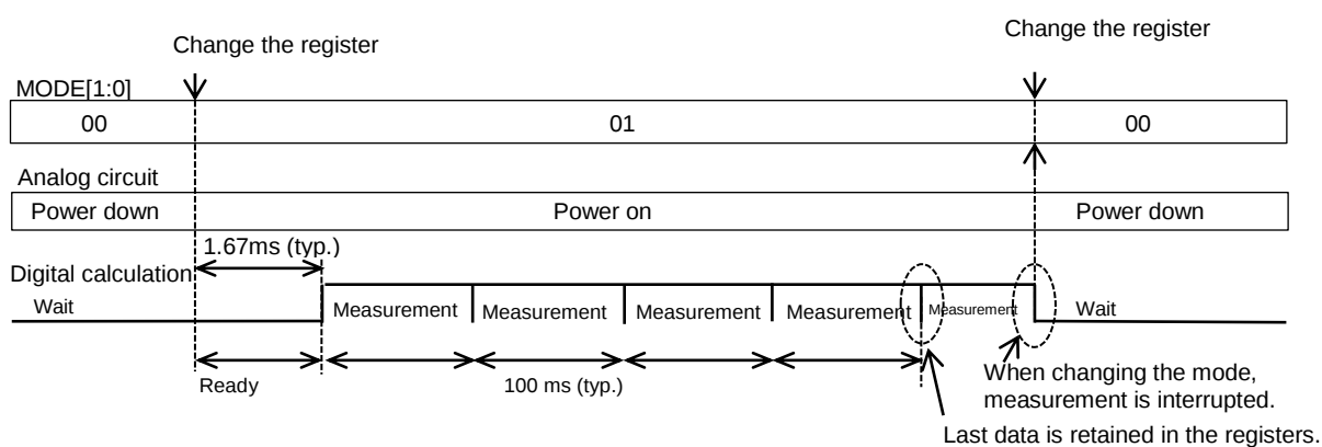
Figure 10.2. Continuous Mode
