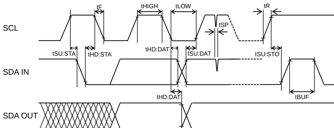
Figure 9.1. Bus Timing
