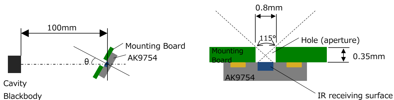
Figure 15.2. Measurement Environment
