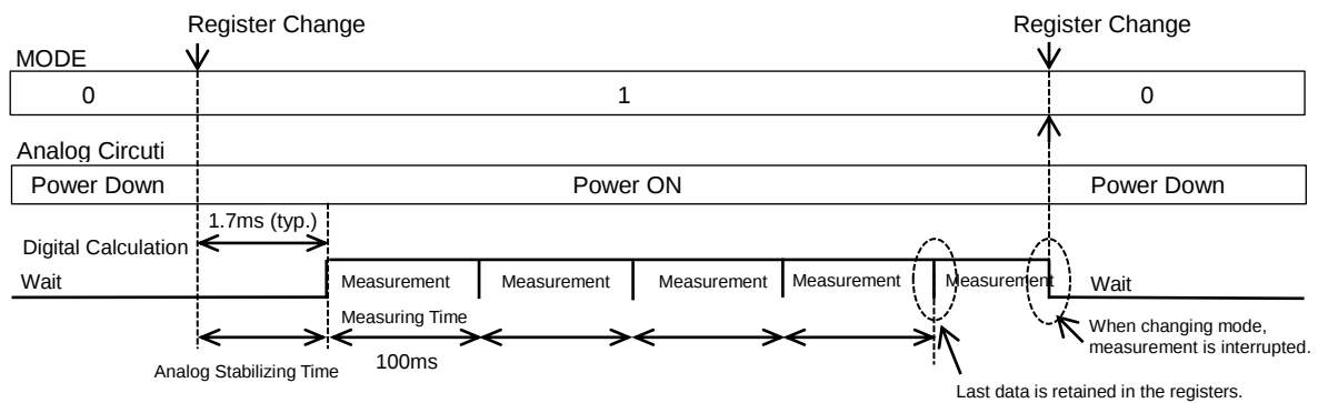
Figure 10.2. Continuous Mode
