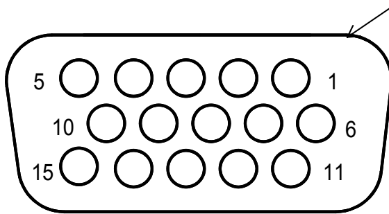
D-sub connector
