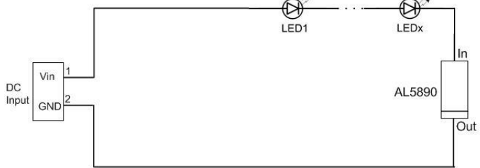
Figure 16. Low Side DC Application
