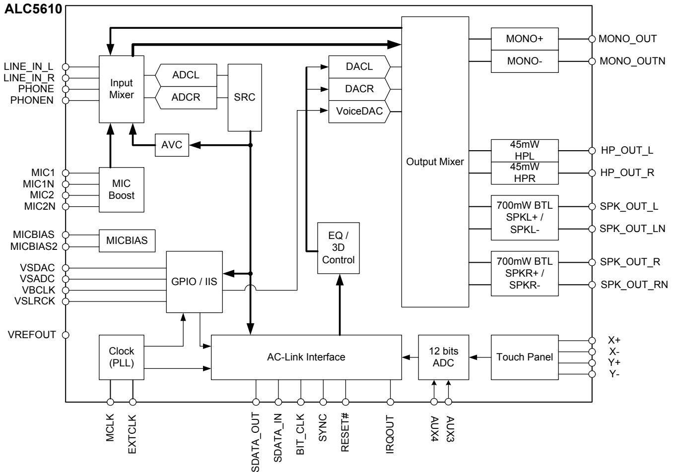
Figure 1. Block Diagram
