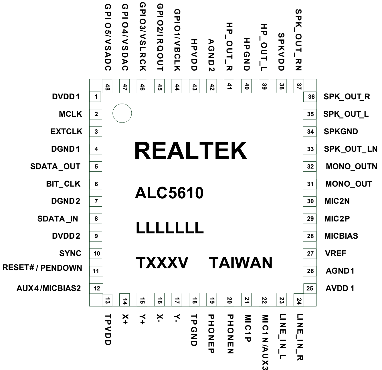
Figure 3. Pin Assignments
