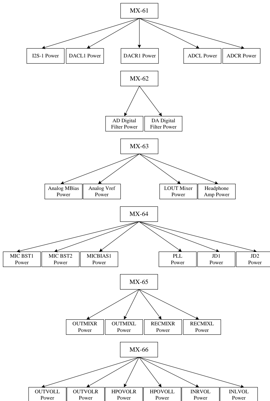
Figure 23. Power Management
