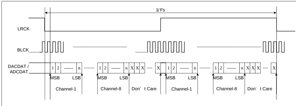
Figure 18. I²S TDM Data Format (BCLK POLARITY=0)
