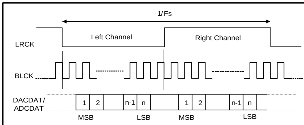
Figure 17. I²S Data Format (BCLK POLARITY=0)
