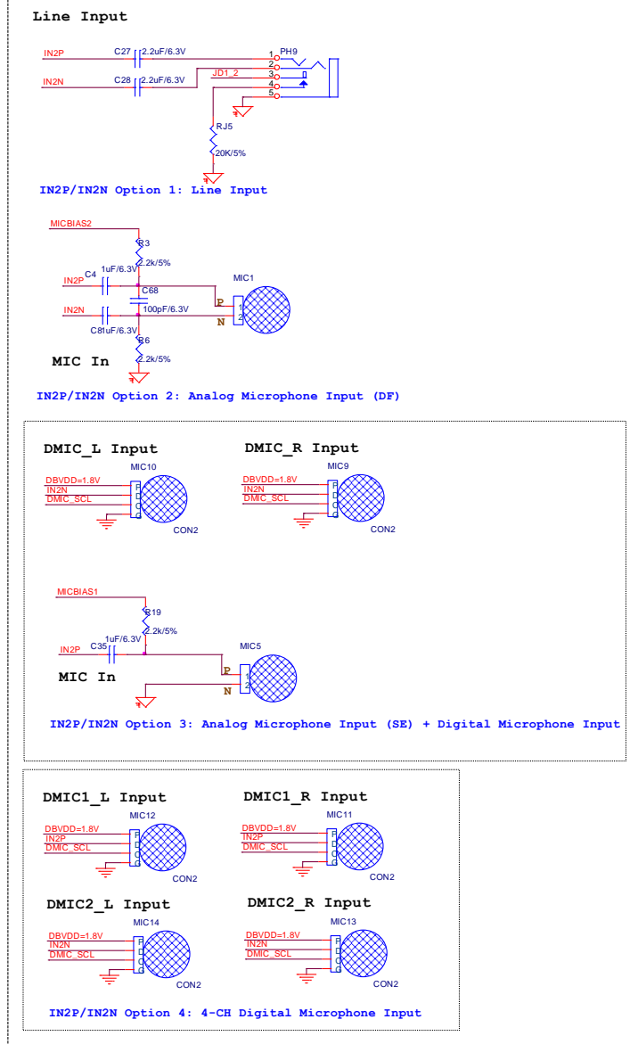
Figure 34. Application Circuit
