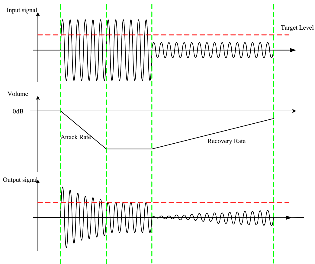
Figure 24. DRC/AGC for Playback/Recording Mode
