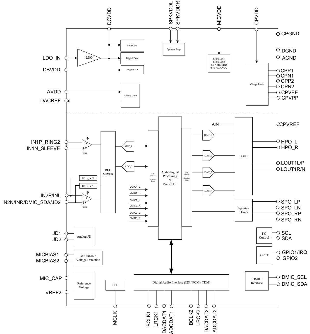
Figure 1. Block Diagram
