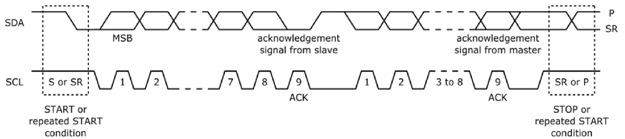
Figure 21. Bit transfer
