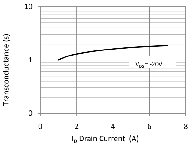
Transconductance
