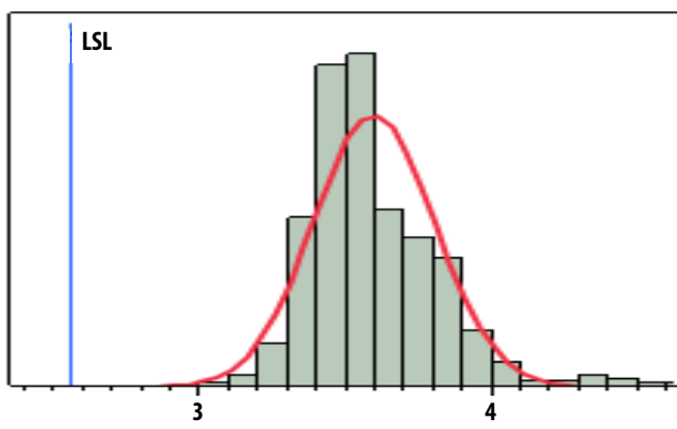
Figure 5. IP1dB, LSL = 2.55 dBm, nominal = 3.5 dBm
