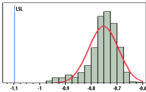
Figure 6. Bypass IL, LSL = 1.1 dB, nominal = 0.75 dB
