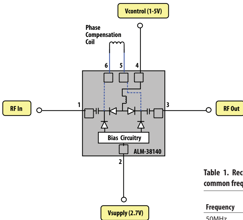
Figure 32. Simplified Schematic
