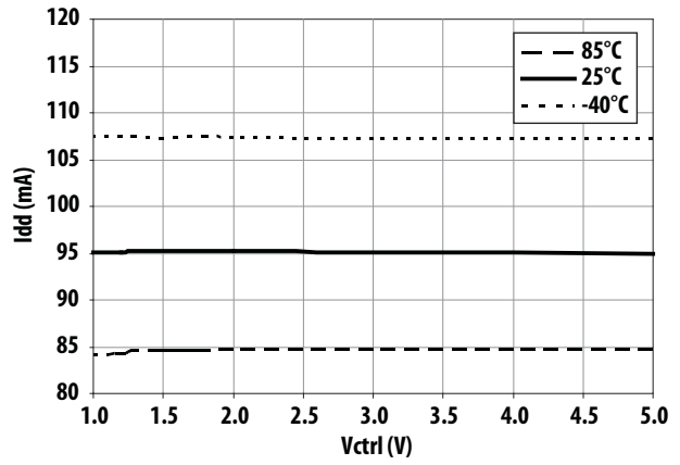
Figure 26. Current ( I_{dd} ) vs Control Voltage and Temperature
