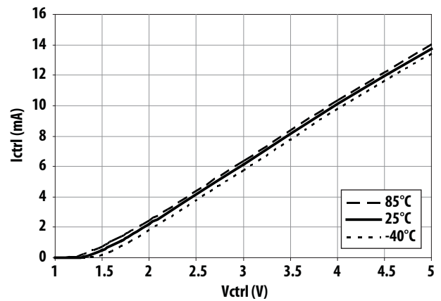
Figure 51. Current ( I_{ctrl} ) vs Control Voltage and Temperature
