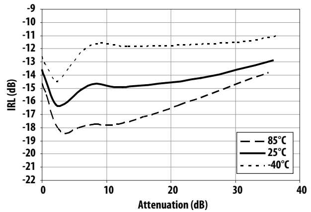
Figure 16. IRL vs Attenuation and Temperature at 1900MHz
