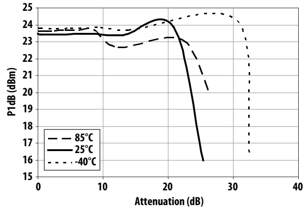
Figure 37. P1dB vs Attenuation and Temperature at 2500MHz
