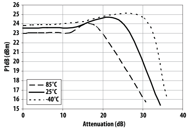
Figure 14. P1dB vs Attenuation and Temperature at 1900MHz
