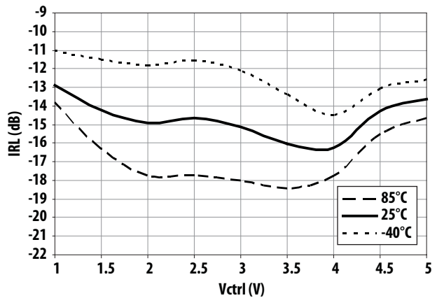
Figure 10. IRL vs Control Voltage and Temperature at 1900MHz
