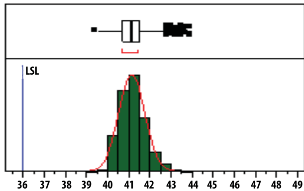
Figure 5. OIP3 at 1900MHz
