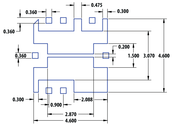
Stencil Outline
