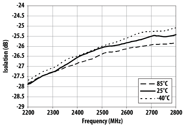
Figure 46. Isolation Frequency and Temperature at V_{ctrl} = 5\text{V}
