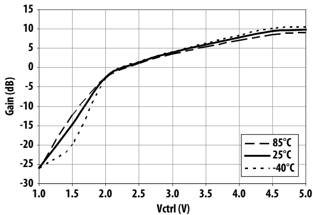
Figure 9. Gain vs Control Voltage and Temperature at 1900MHz
