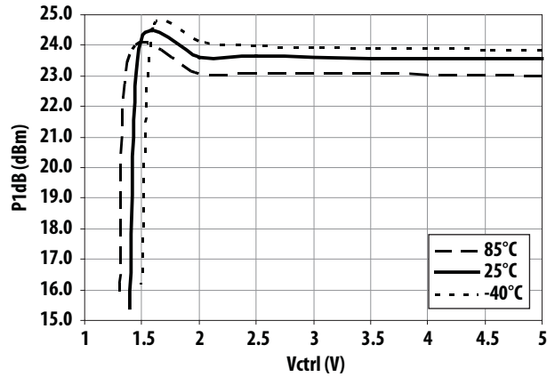
Figure 8. P1dB vs Control Voltage and Temperature at 1900MHz
