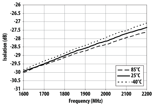
Figure 23. Isolation Frequency and Temperature at V_{ctrl} = 5\text{V}
