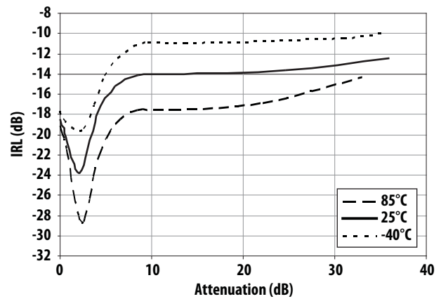
Figure 39. IRL vs Attenuation and Temperature at 2500MHz
