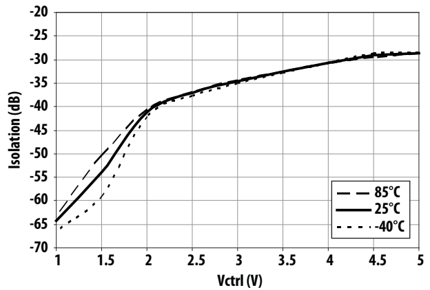
Figure 12. Isolation vs Control Voltage and Temperature at 1900MHz
