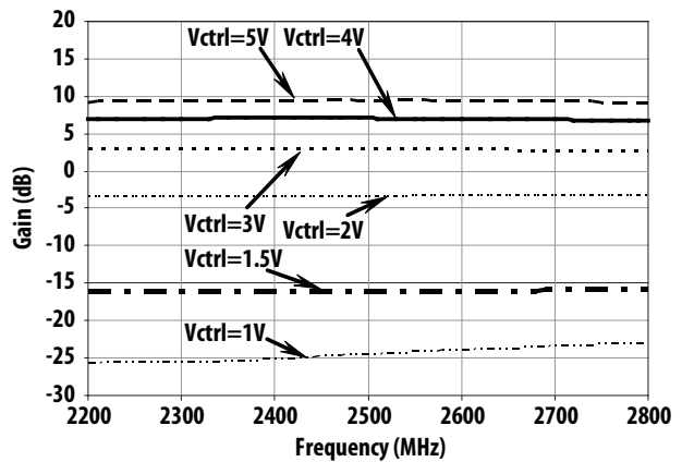
Figure 47. Gain vs Frequency and Control Voltage
