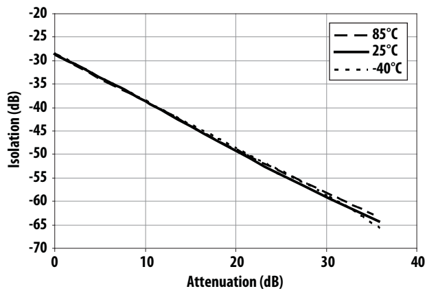
Figure 17. Isolation vs Attenuation and Temperature at 1900MHz
