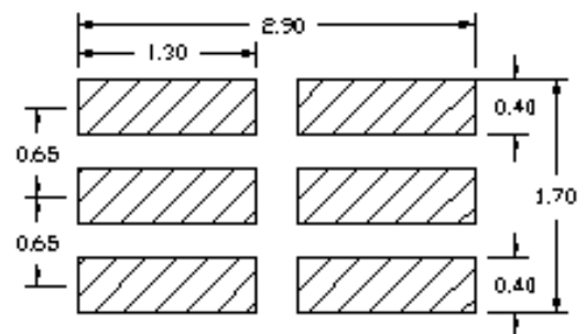
soldering pattern
