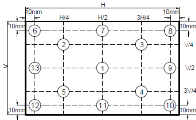
Figure 6 Measurement Locations
