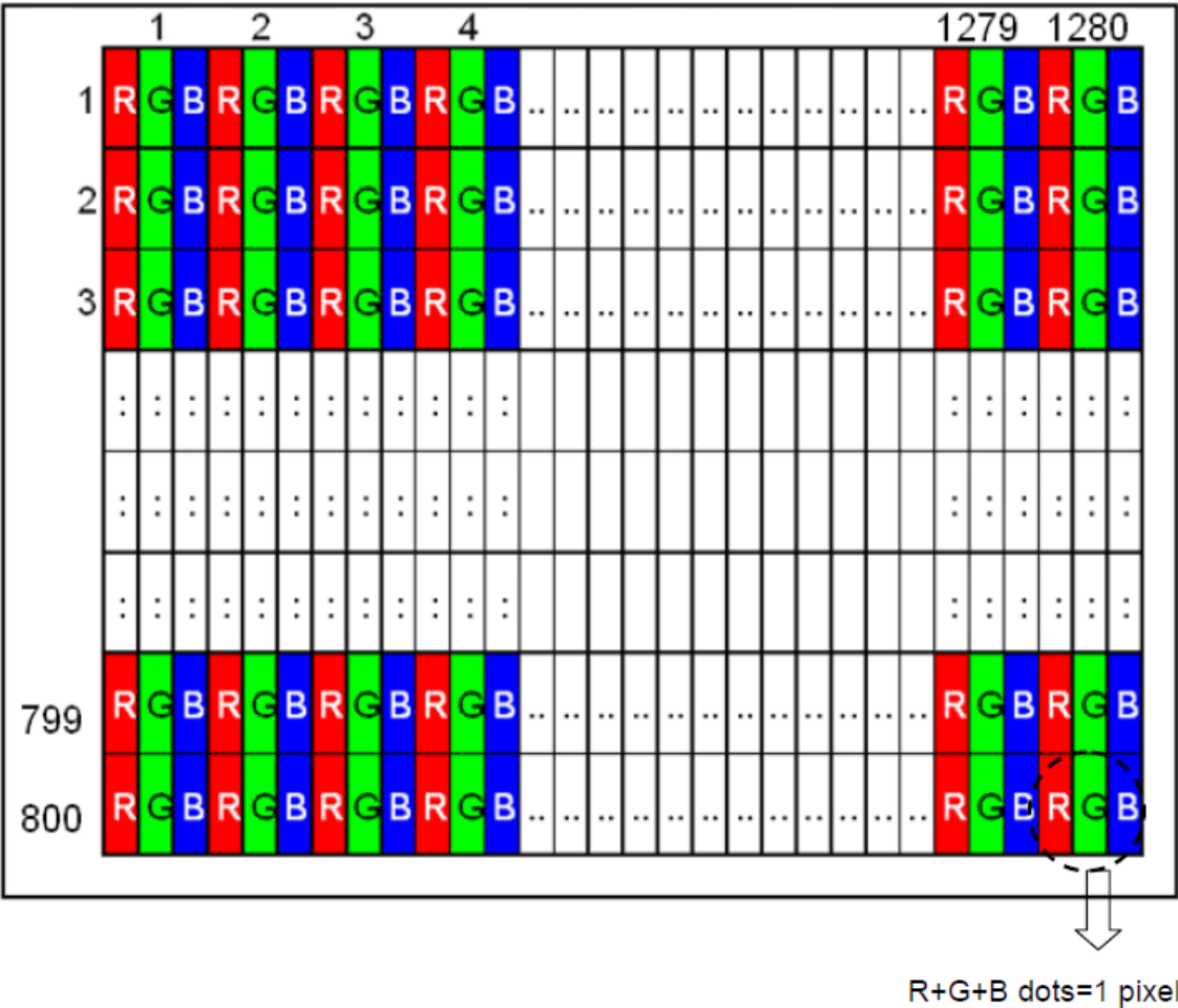
Figure 2 Pixel Format
