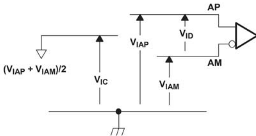
Figure 2. Voltage Definitions
