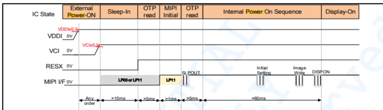
Figure 15 Power-On Sequence
