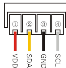
Figure 4: AM2321 wiring diagram
