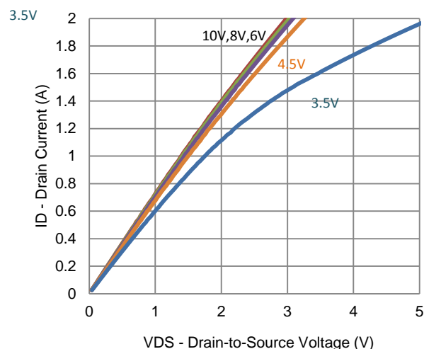
5. Output Characteristics
