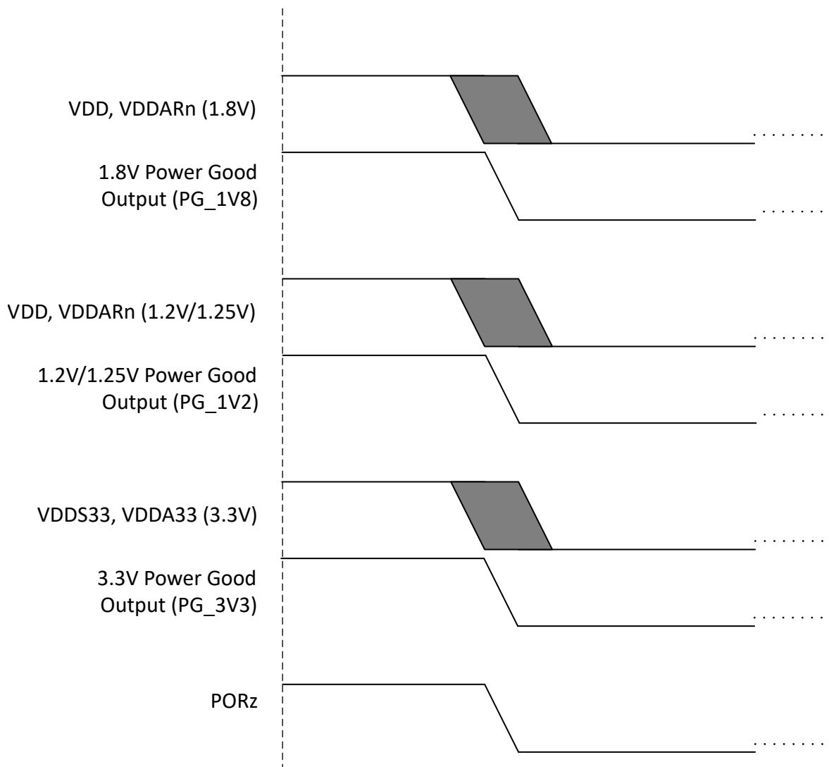
Figure 6-3. Power-Down Sequencing
