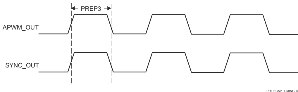
Figure 6-80. PRU-ICSS ECAP Switching Characteristics
