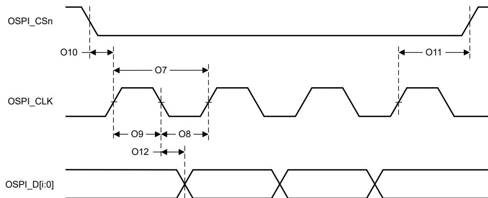
Figure 6-58. OSPI Switching Characteristics – PHY SDR
