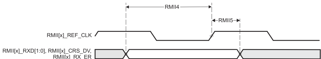
Figure 6-14. CPSW RMII[x]_RXD[1:0], RMII[x]_CRS_DV, RMII[x]_RX_ER Timing Requirements – RMII Mode
