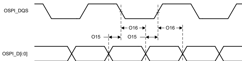
Figure 6-59. OSPI Timing Requirements – PHY DDR with External Board Loopback or DQS
