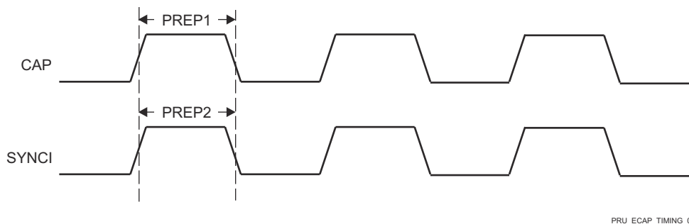
Figure 6-79. PRU-ICSS ECAP Timing
