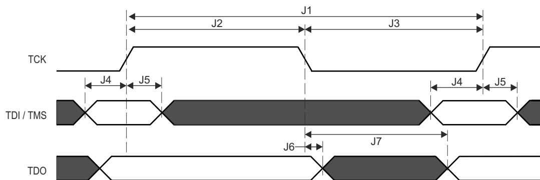
Figure 6-87. JTAG Timing Requirements and Switching Characteristics
