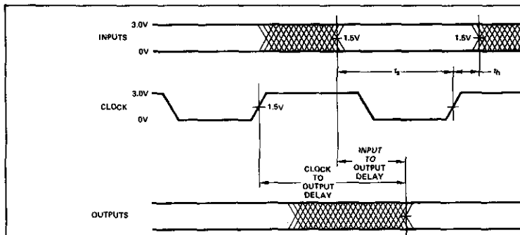
Figure 2. Switching Waveforms.
