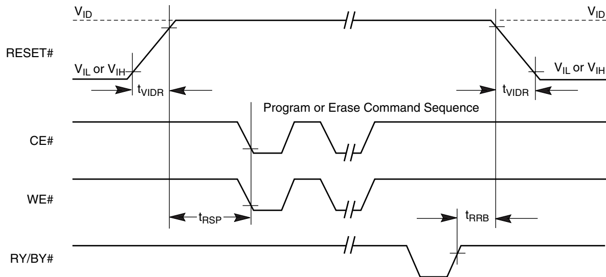
Figure 22. Temporary Sector Unprotect Timing Diagram
