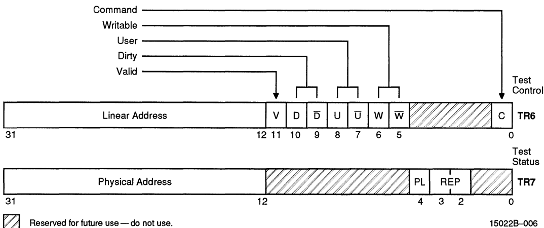
Figure 6. Test Registers
