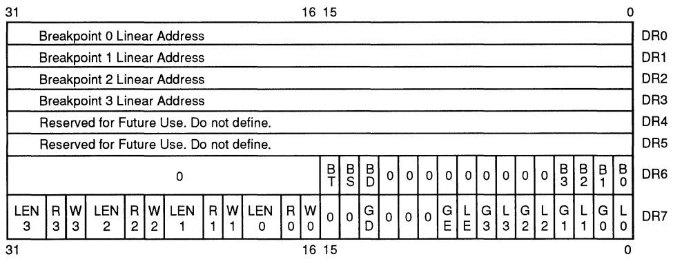
Figure 13. Debug Registers
