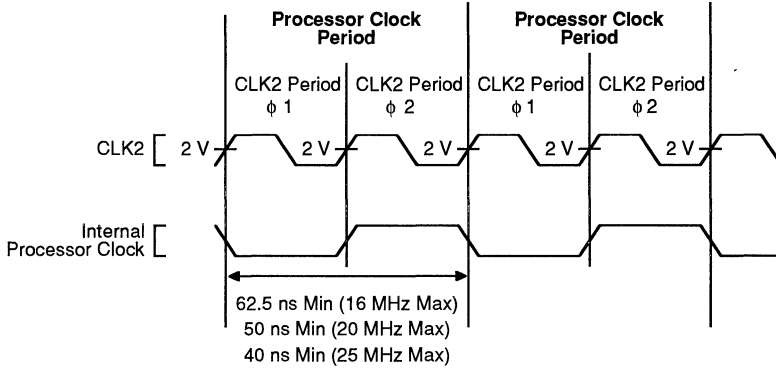
Figure 23. CLK2 Signal and Internal Processor Clock
