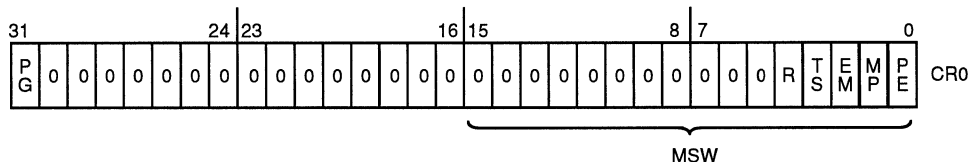
Figure 5. Control Register 0
