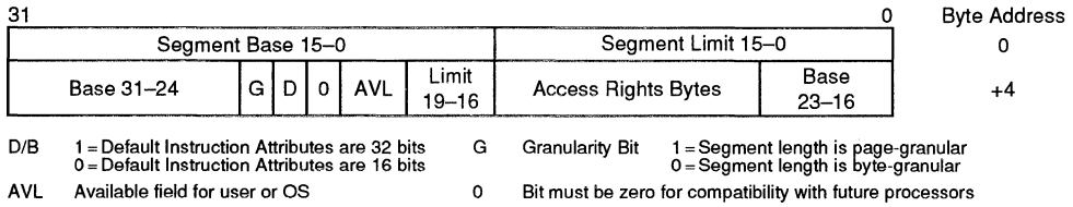
Figure 12. Code and Data Descriptors
