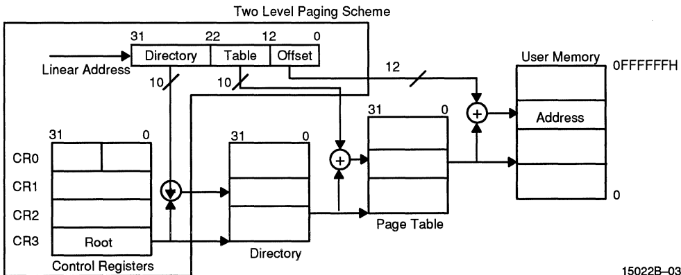
Figure 17. Paging Mechanism
