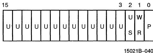
Figure 37. Page Fault Error Code Format
