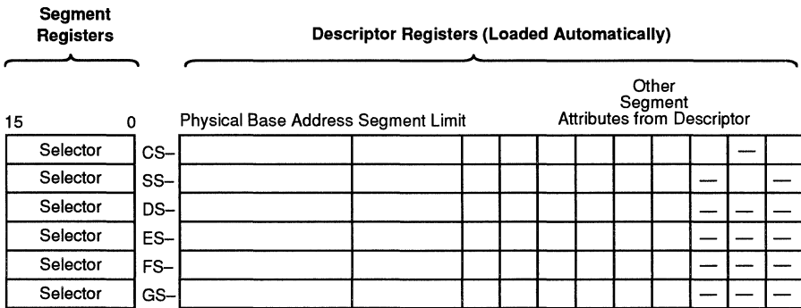
Figure 3. Flags Registers
