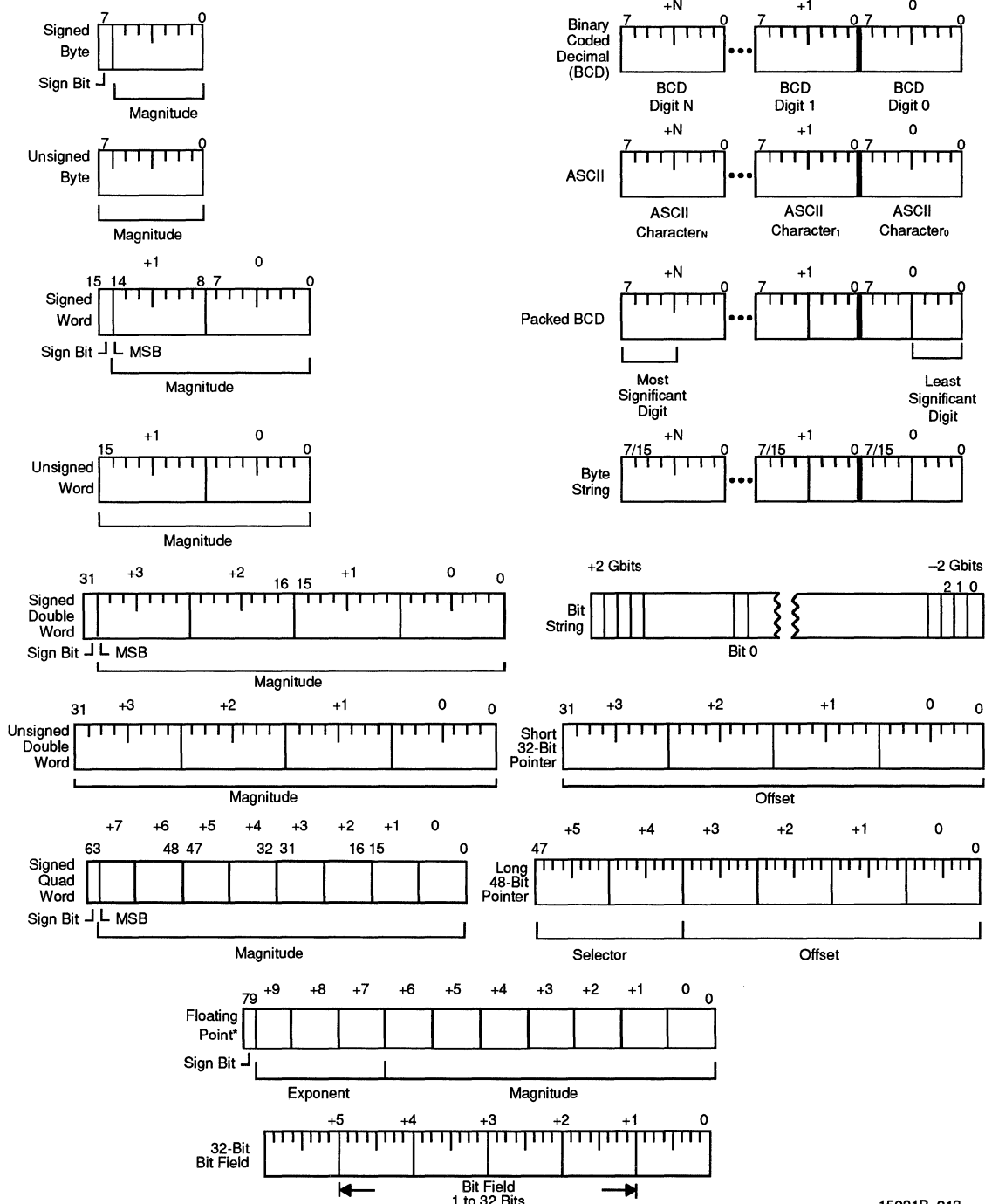
Figure 5. Am386SX/SXL Microprocessor Supported Data Types
