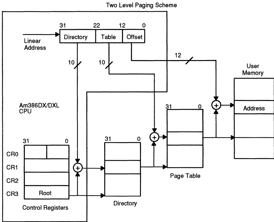
Figure 33. Paging Mechanism
