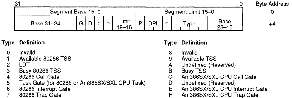
Figure 13. System Descriptors
