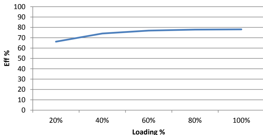
AM3T-1205S-RVZ Efficiency vs. Loading
