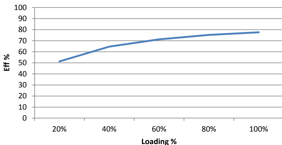
AM3T-4815S-VZ Efficiency vs. Loading
