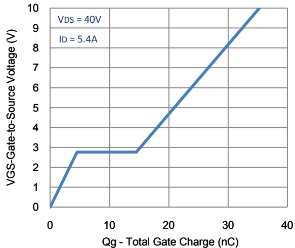
7. Gate Charge
