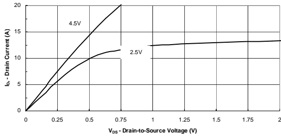
Output Characteristics
