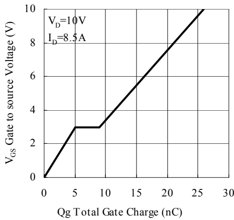
Figure 7. Gate Charge Characteristic
