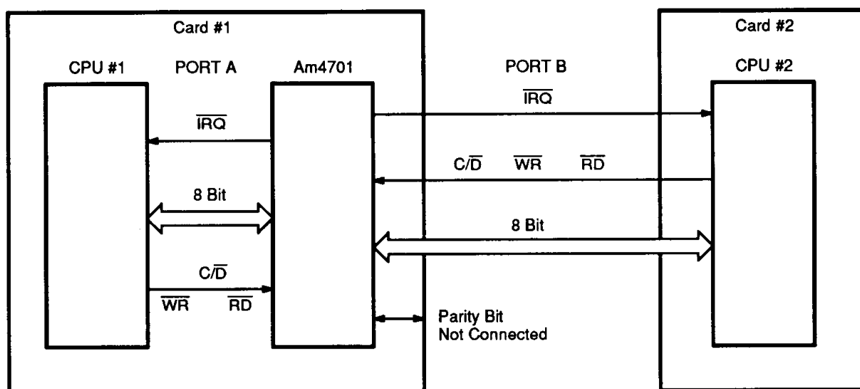
Figure 1. CPU-CPU Communication
