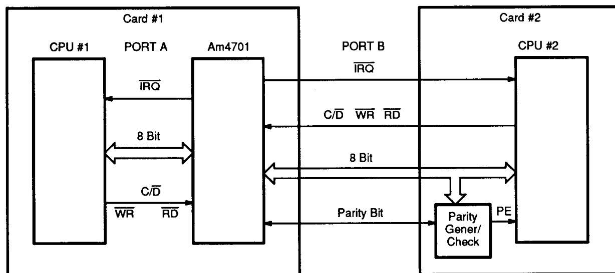
Figure 2. CPU-CPU Communication with Parity
