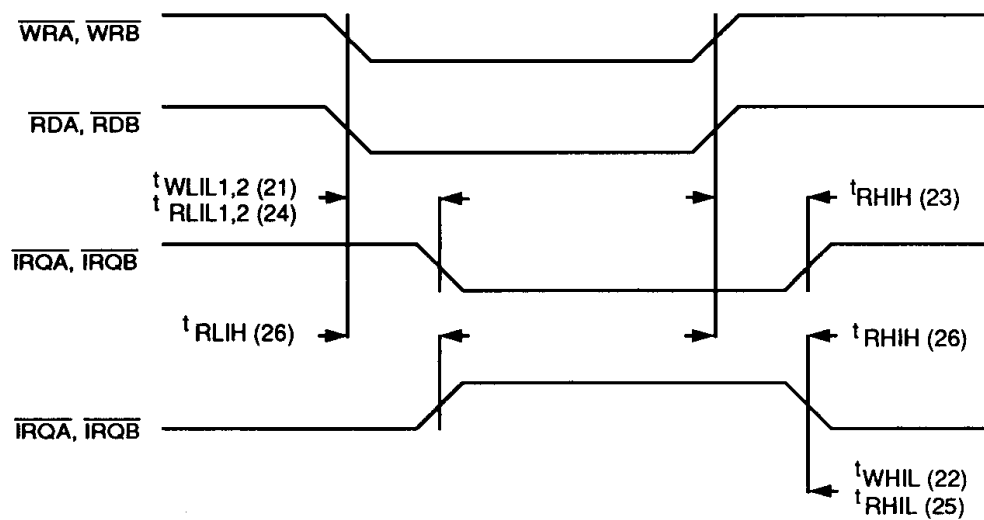
IRQ Timing
