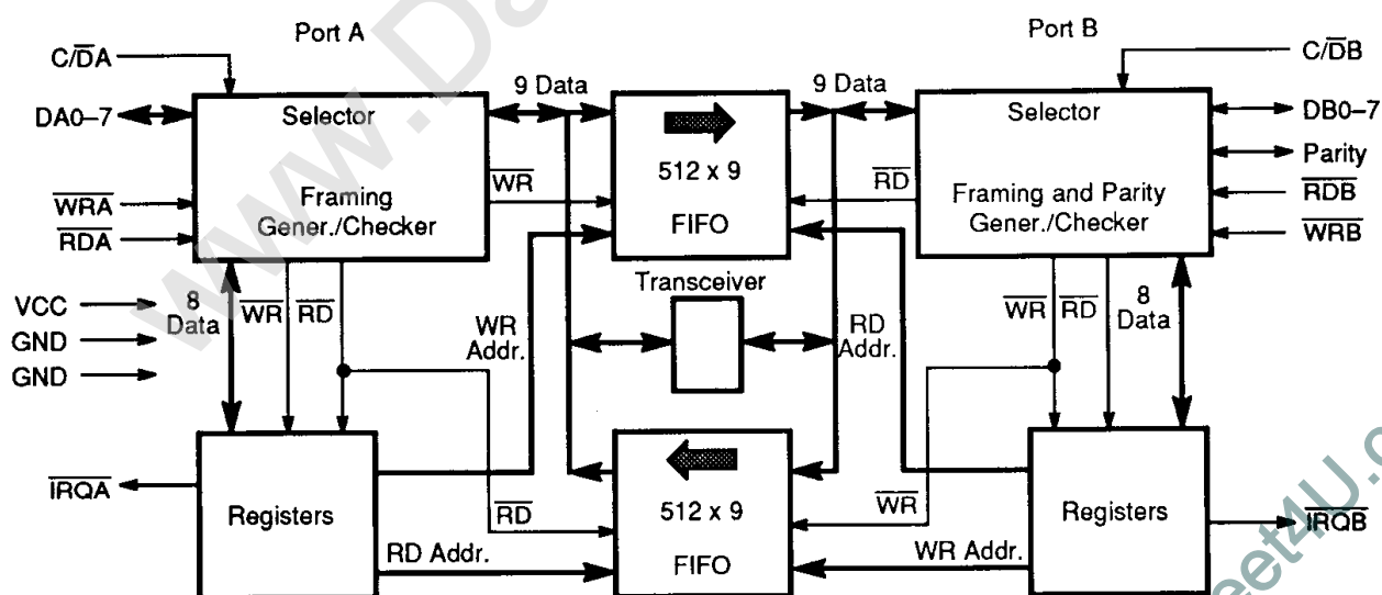
2-512 x 9 BIFIFO
