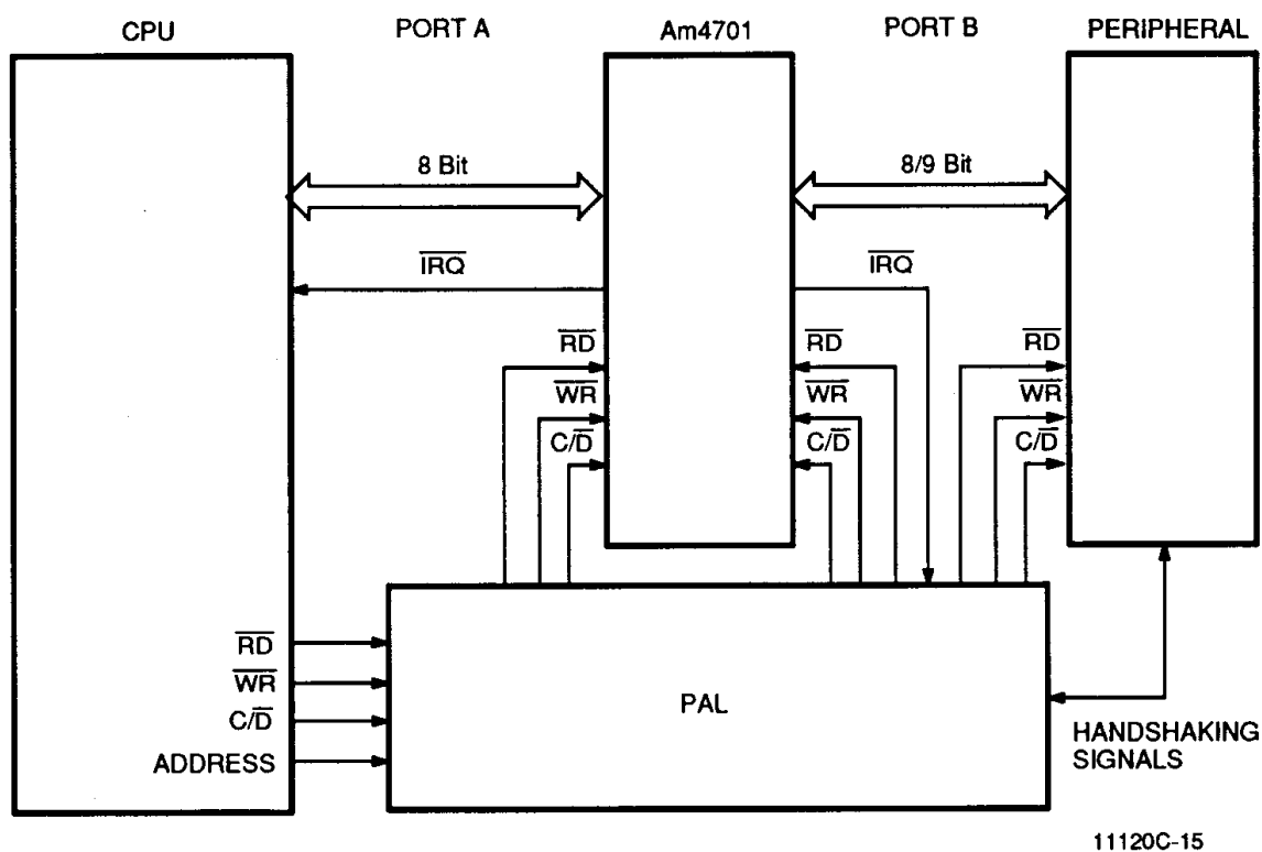
Figure 3. CPU-Peripheral Communication with Bypass
