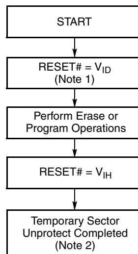
Figure 1. Temporary Sector Unprotect Operation
