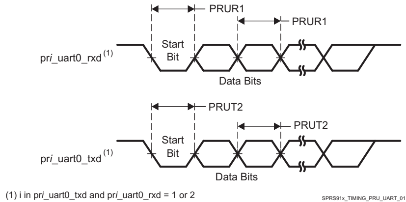
Figure 5-128. PRU-ICSS UART Timing
