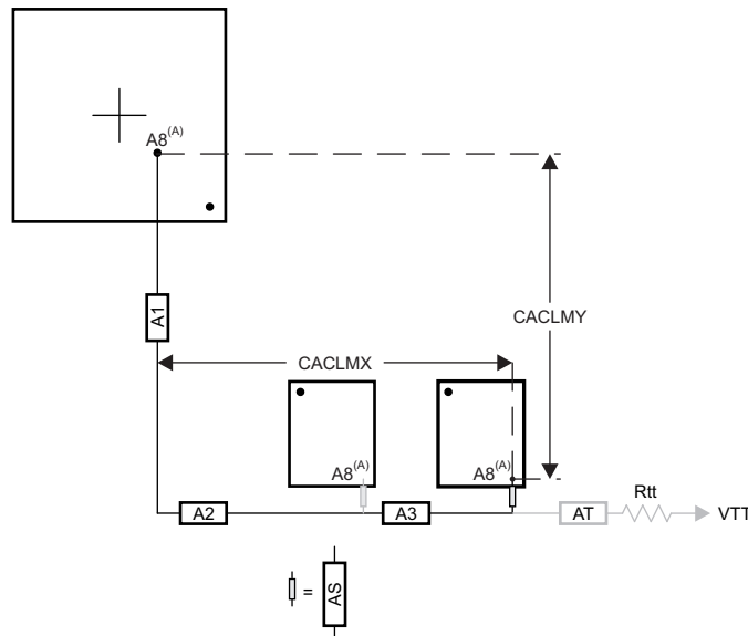
Figure 7-26. CACLML for Four Address Loads on One Side of PCB
