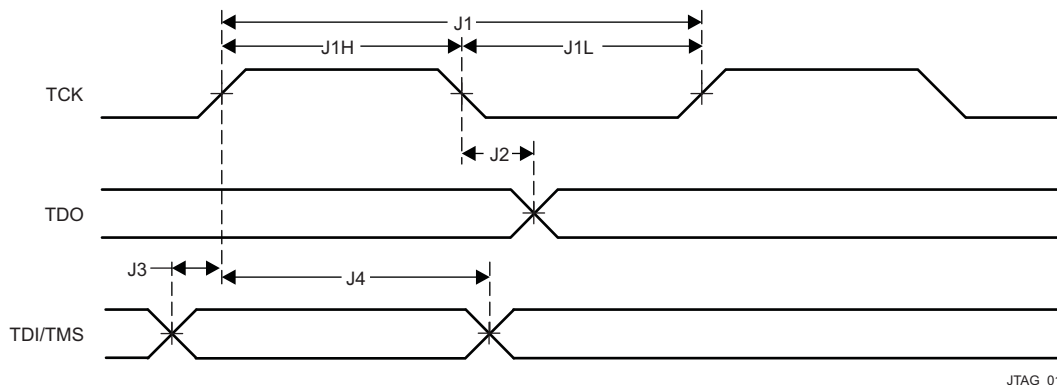
Figure 5-129. JTAG Timing
