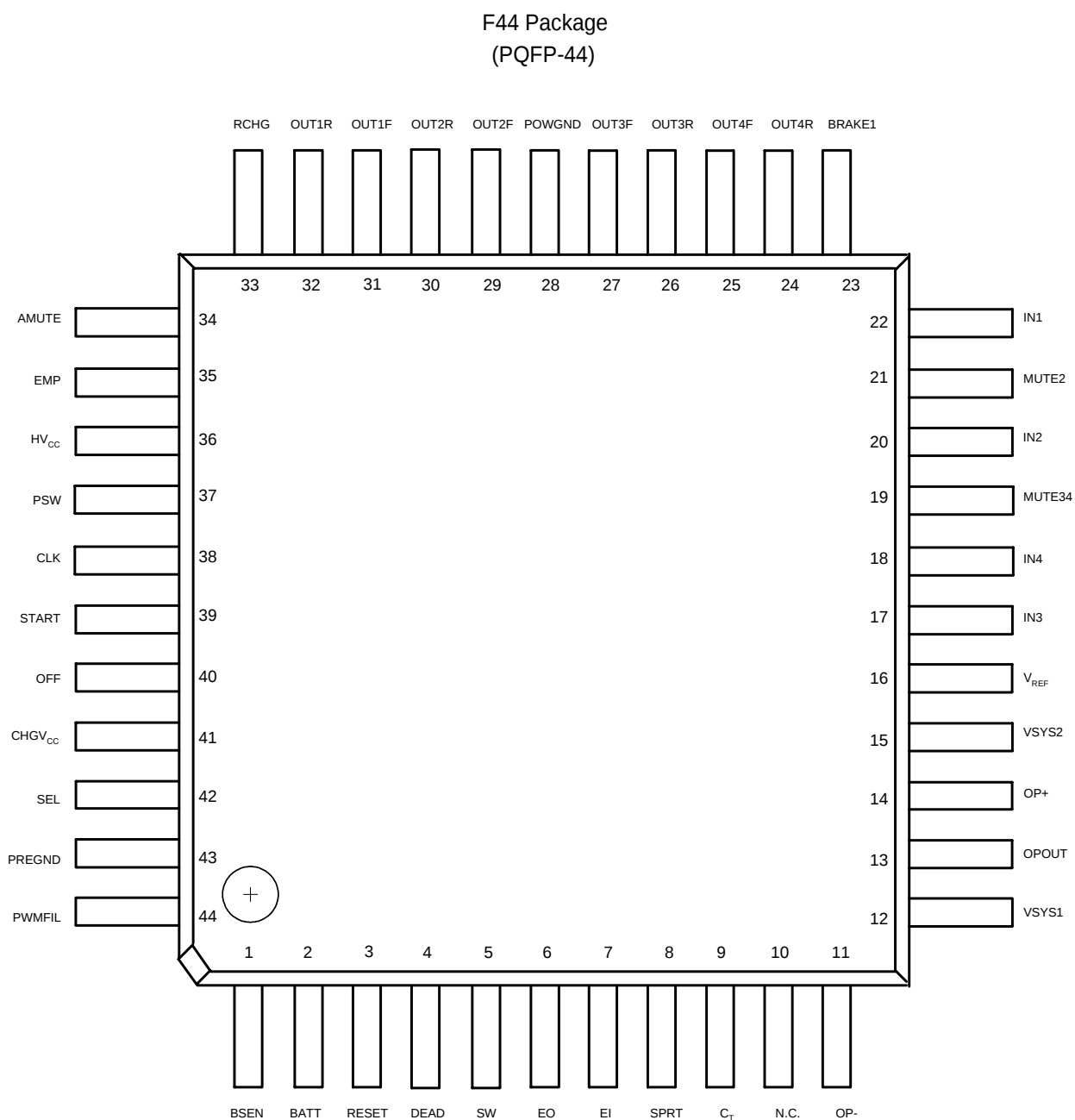
Figure 2. Pin Configuration of AM5901A (Top View)
