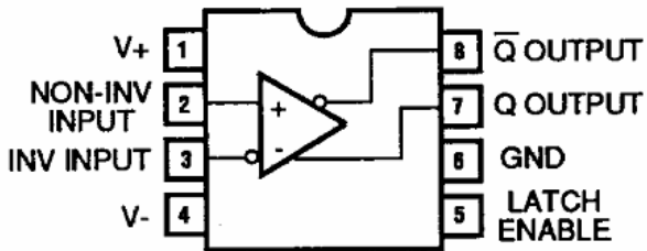
Dual In-Line P-8-1
