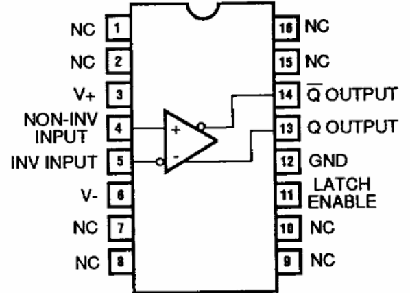
Dual In-Line D-16-1
