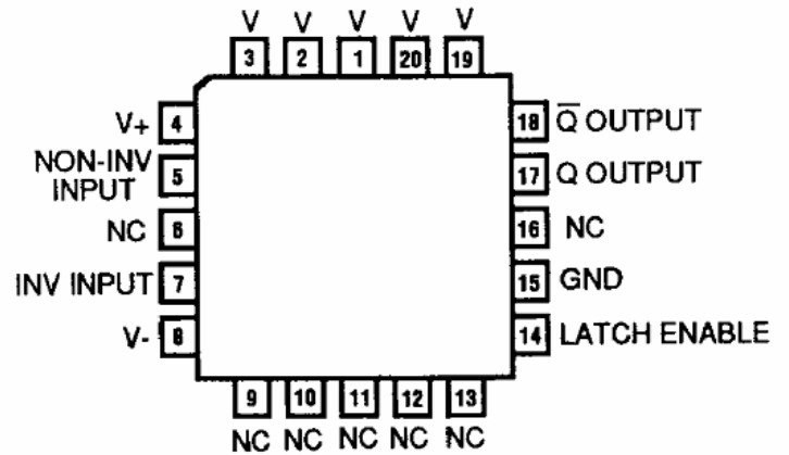
Leadless Chip-Pak L-20-1
