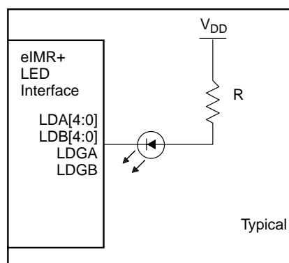
Figure 1. Visual Monitoring Application—Direct LED Drive
