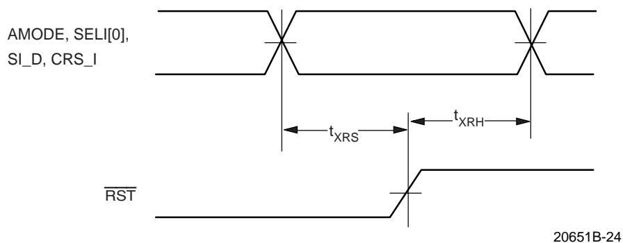
Figure 19. Mode Initialization
