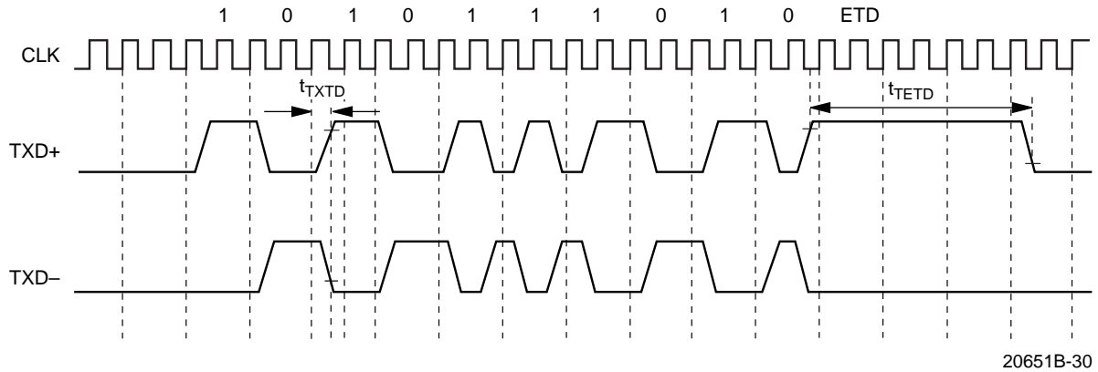
Figure 25. TP Ports Output Timing Diagram
