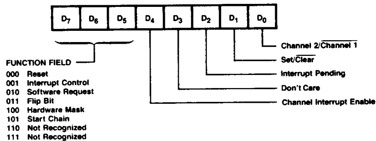
Figure 19. Command Register
