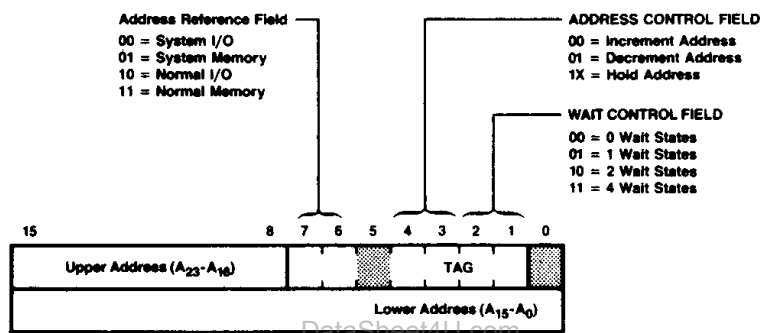
Figure 4. Address Registers A and B
