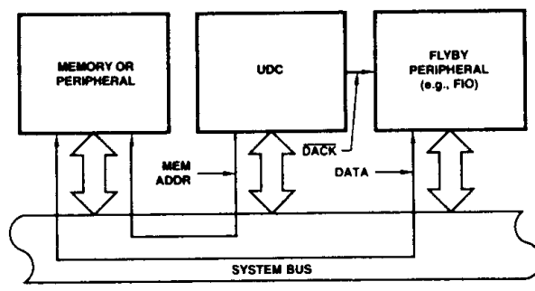
Figure 15. Configuration of Flyby Transaction
