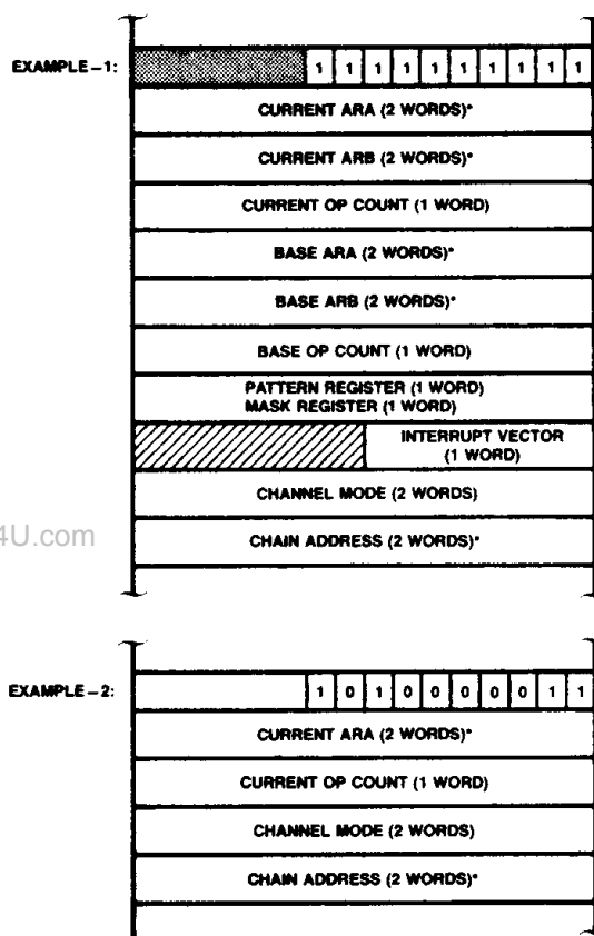
Figure 12. Examples of Chain Control Table
