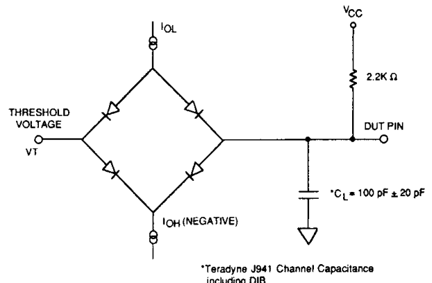
B. Open-Drain Dynamic Load
