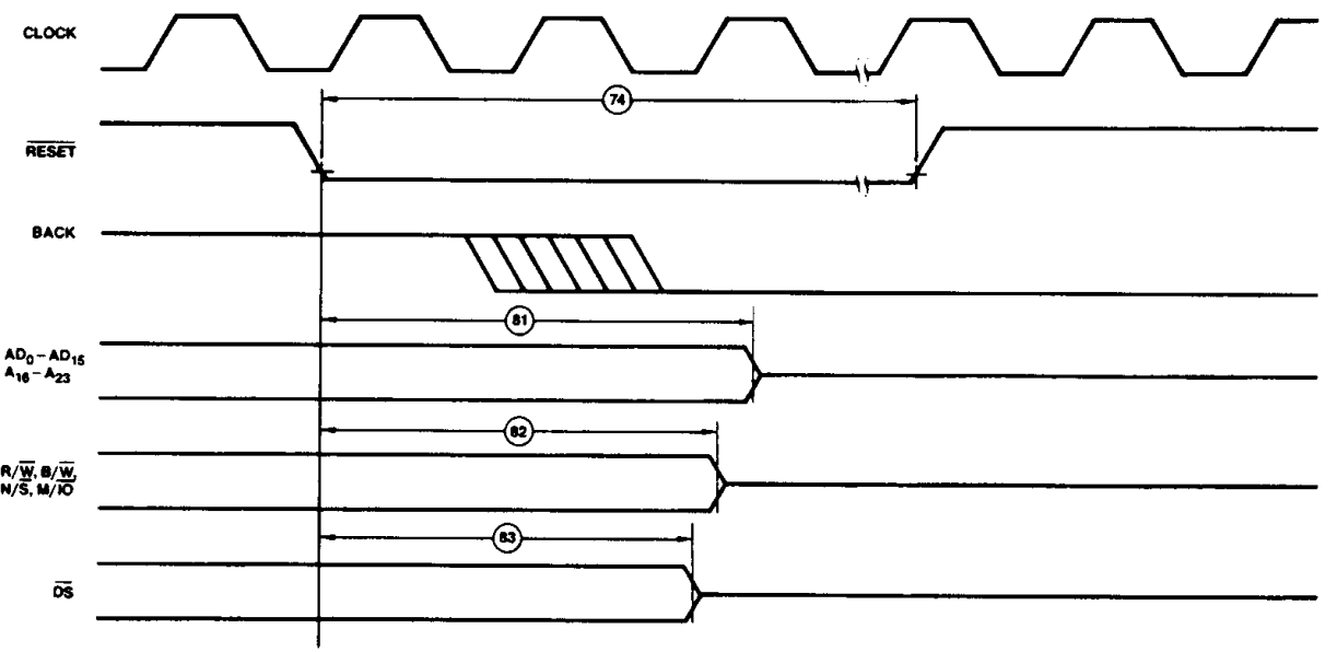
TIMING DIAGRAM 12. Reset Timing
