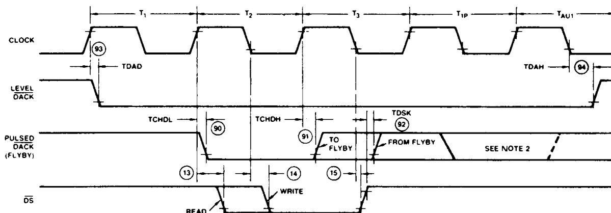
TIMING DIAGRAM 3. DACK Timing
