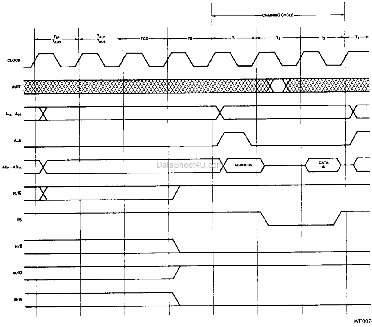
TIMING DIAGRAM 14. Timing During Chaining
