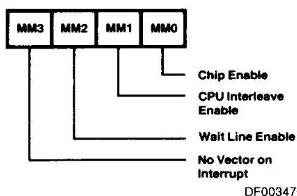
Figure 3. Master Mode Register
