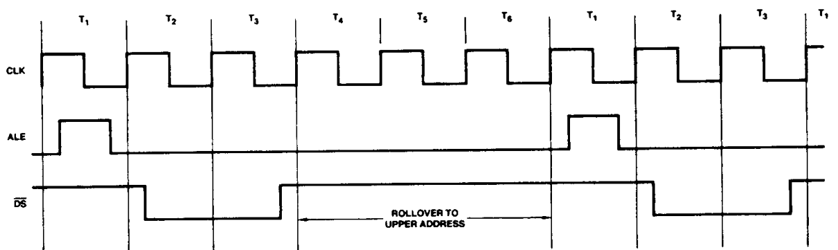
TIMING DIAGRAM 10. Upper Address Rollover Timing
