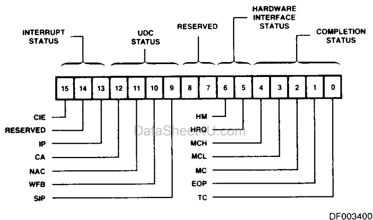
Figure 5. Status Register
