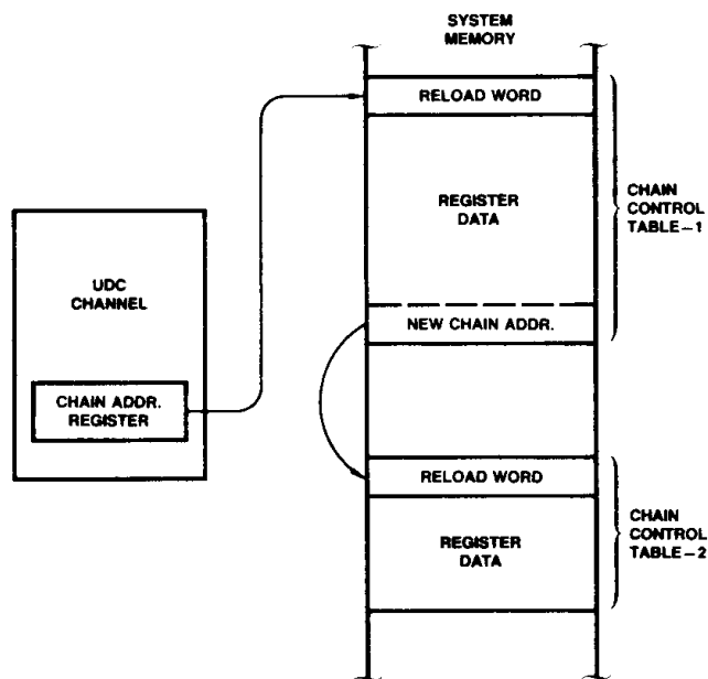
Figure 10. Chaining and Chain Control Tables
