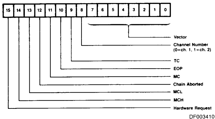
Figure 6. Interrupt Save Register
