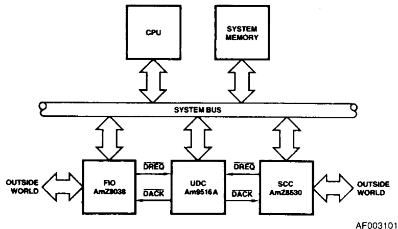
Figure 1. UDC Configurations
