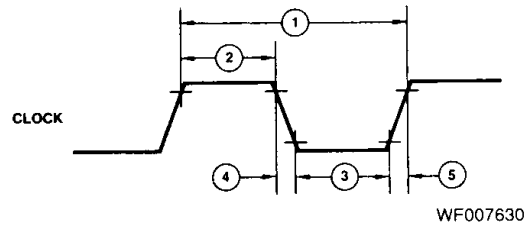
TIMING DIAGRAM 14. Timing During Chaining
