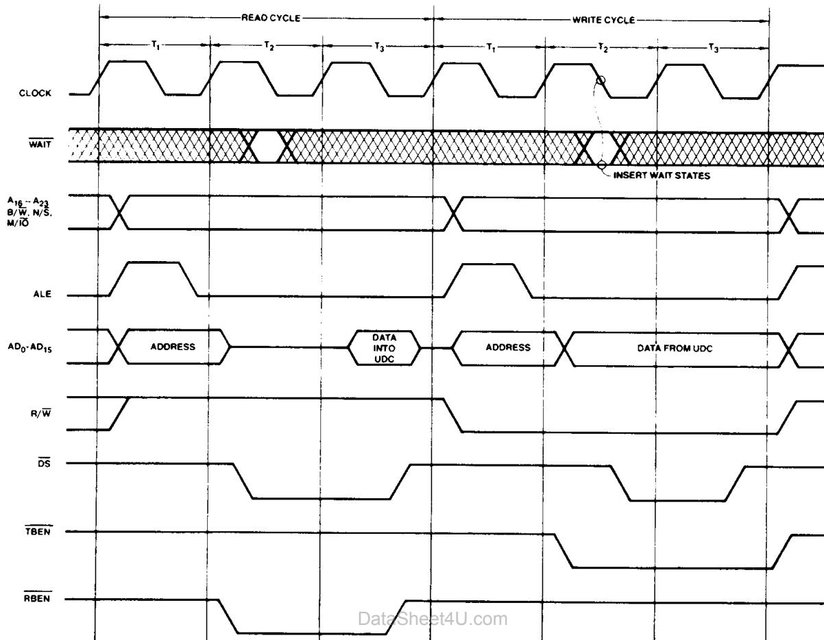
TIMING DIAGRAM 5. Flowthru Transactions
