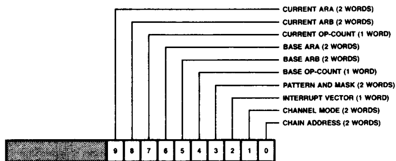
Figure 11. Reload Word/Chain Control Register
