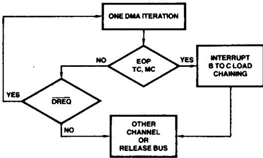
(b) Demand Operation when Software Requesting
