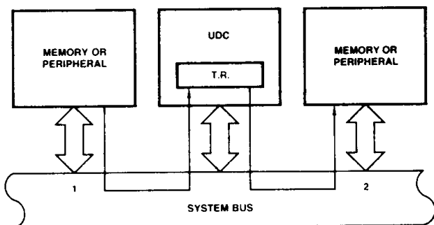
Figure 14. Configuration of Flowthru Transaction
