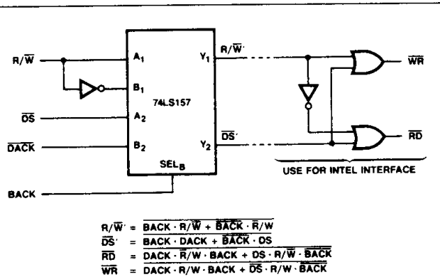
Figure 16. Flyby Peripheral Interface
