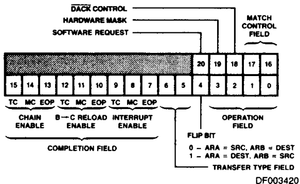
Figure 7. Channel Mode Register
