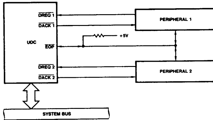
Figure 17. \overline{EOP} Connection
