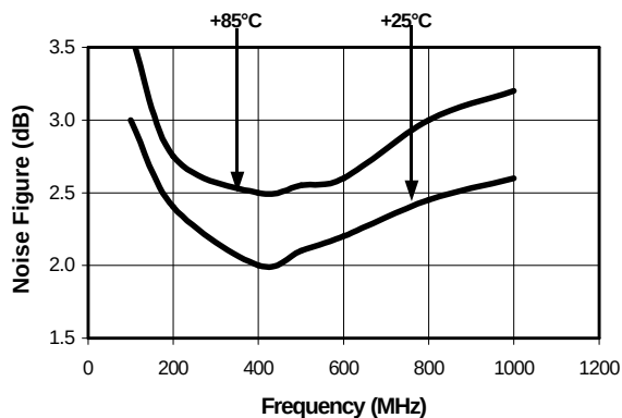
Noise Figure
