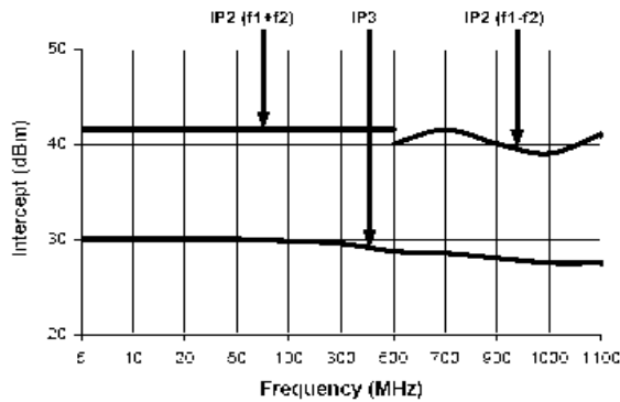
Intermodulation Intercept
