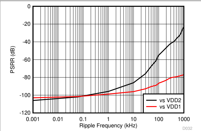
Figure 7-30. Power-Supply Rejection Ratio vs Ripple Frequency
