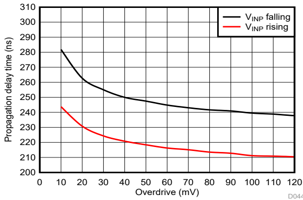
Figure 6-47. Cmp2 Propagation Delay vs Overdrive
