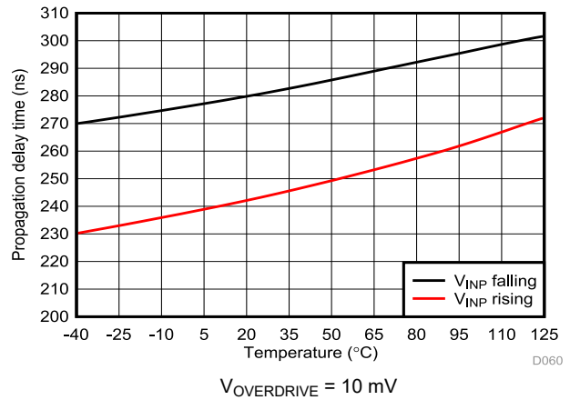
Figure 6-50. Cmp3 Propagation Delay vs Temperature
