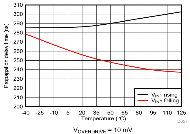
Figure 6-52. Cmp0 Propagation Delay vs Temperature
