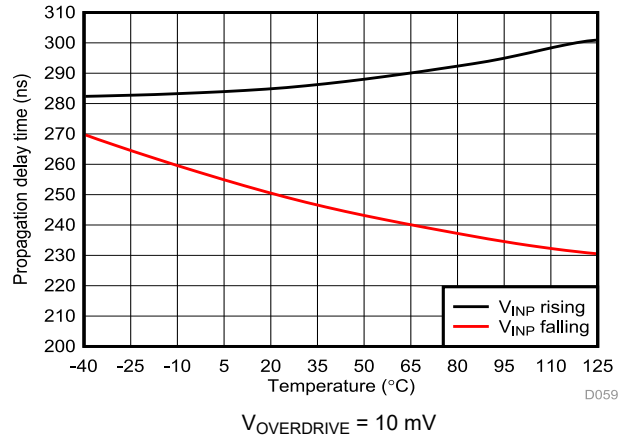
Figure 6-48. Cmp2 Propagation Delay vs Temperature
