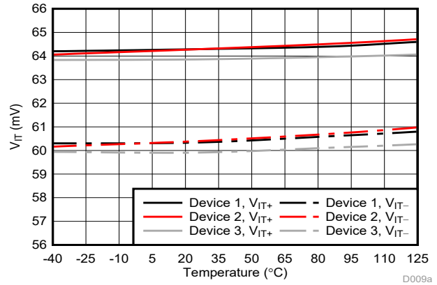
Figure 6-6. Cmp2 Trip Threshold vs Temperature
